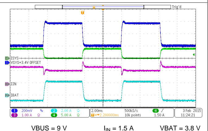
51. Charge Disable
