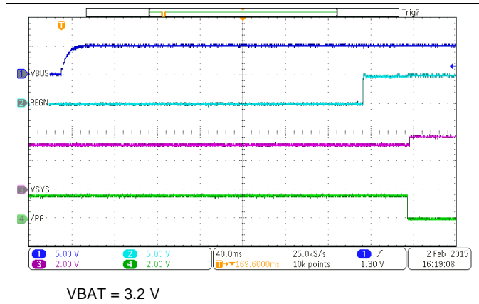
48. Power Up with Charge Disabled
