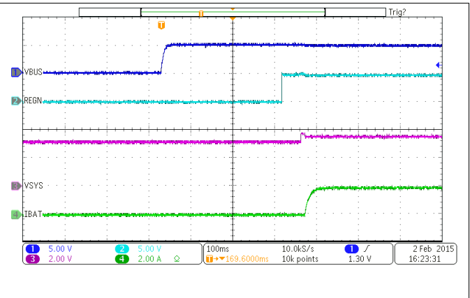
49. Power Up with Charge Enabled
