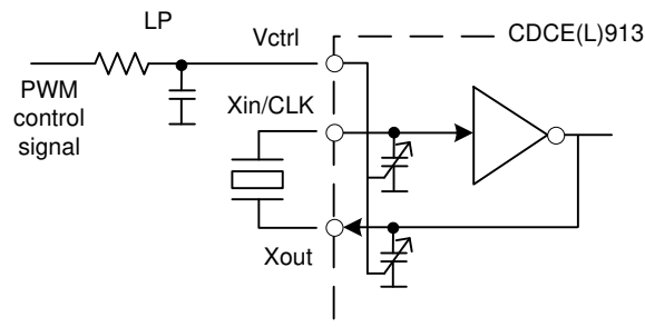
図 8-6. Frequency Adjustment Using PWM Input to the VCXO Control
