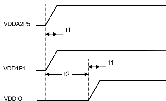
図 8-7. Two-Supply Sequence Diagram
