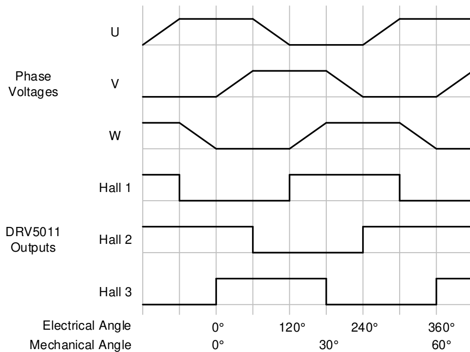
FIG 13. Phase Voltages and Hall Signals for 3-Phase BLDC Motor
