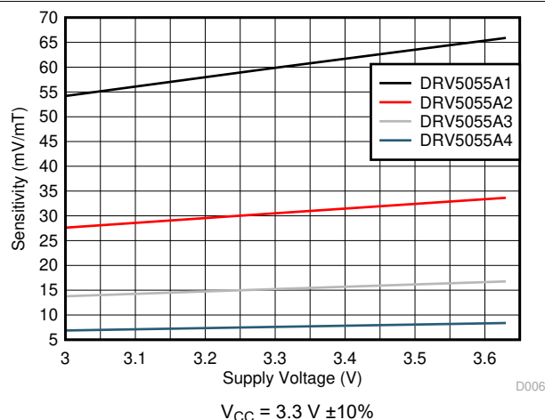
図 5-9. Sensitivity vs Supply Voltage
