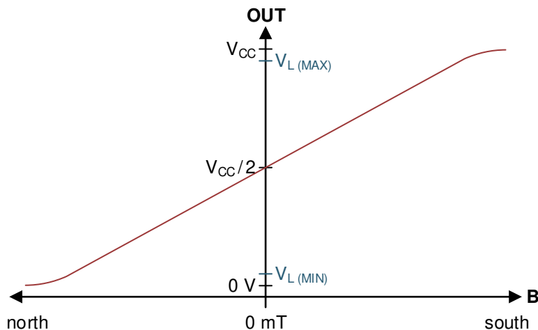
図 6-3. Magnetic Response
