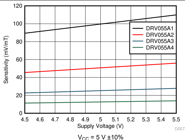
図 5-10. Sensitivity vs Supply Voltage
