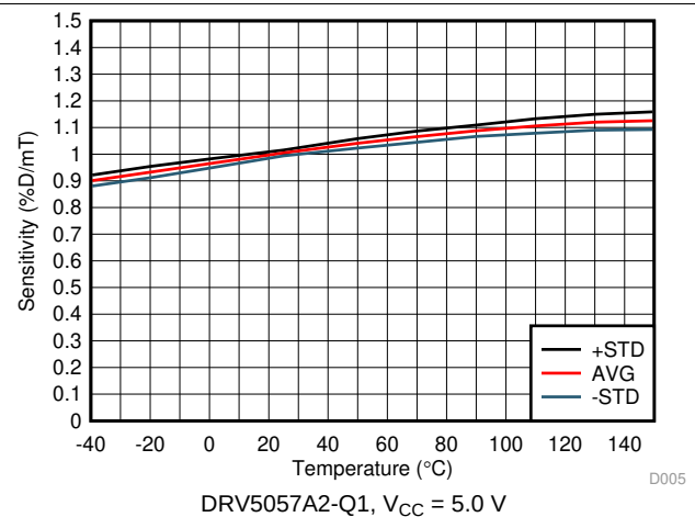
図 6. Sensitivity vs Temperature
