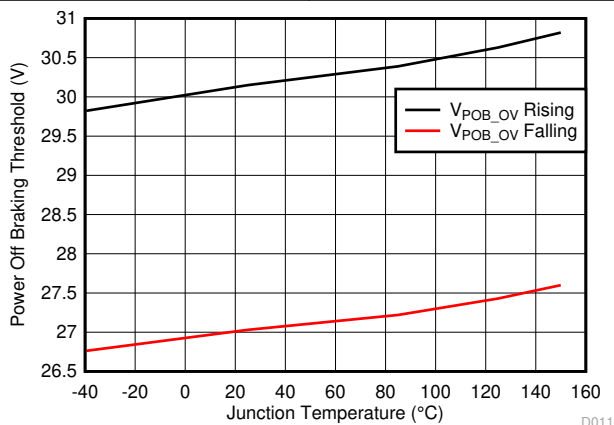
6-12. Power Off Braking Threshold
