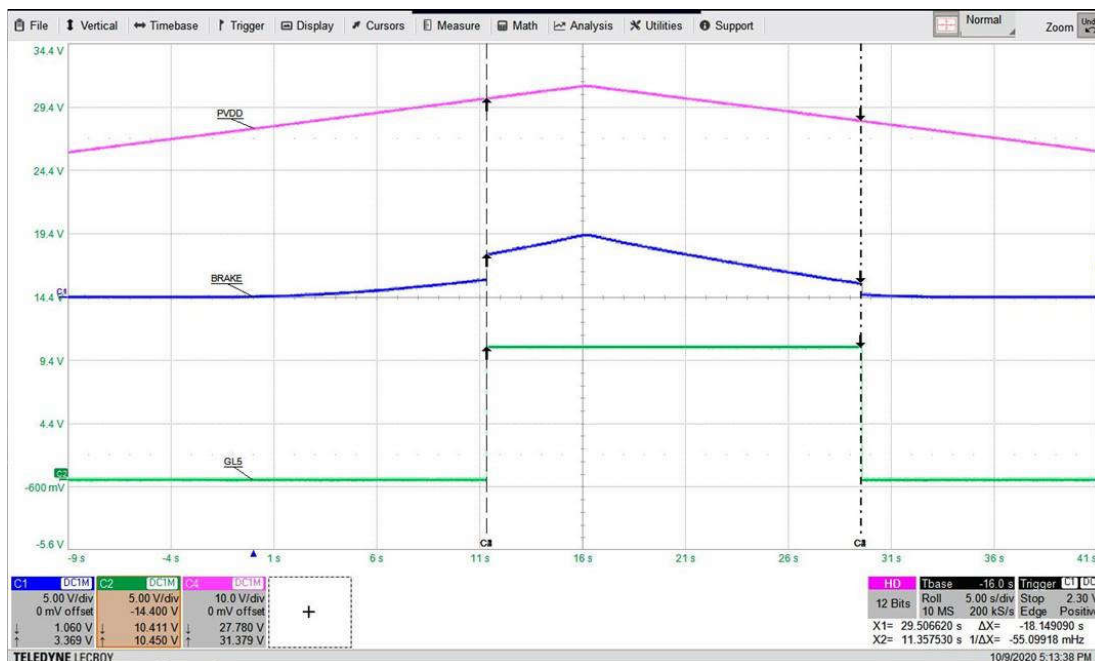
図 9-6. Power Off Braking Low-Side Driver Response
