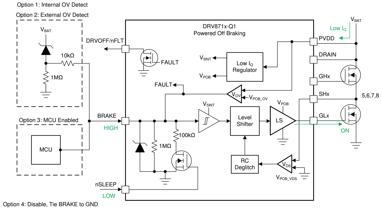
図 7-28. Powered Off Braking
