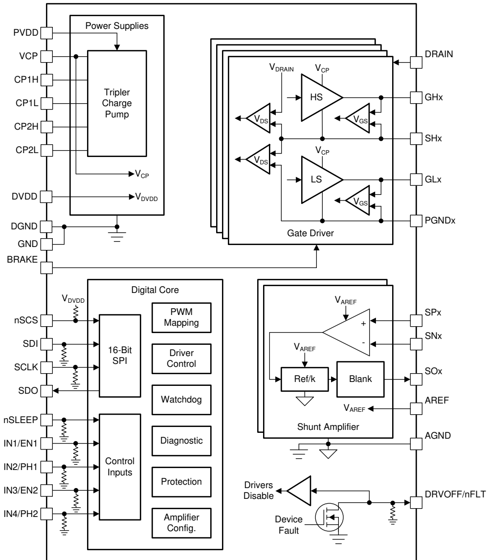
7-2. Block Diagram for DRV8714S-Q1 RVJ Package
