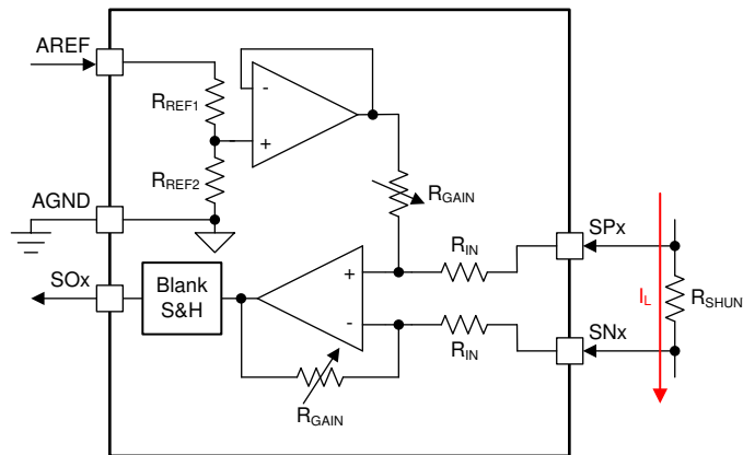
図 7-17. Amplifier Simplified Block Diagram
