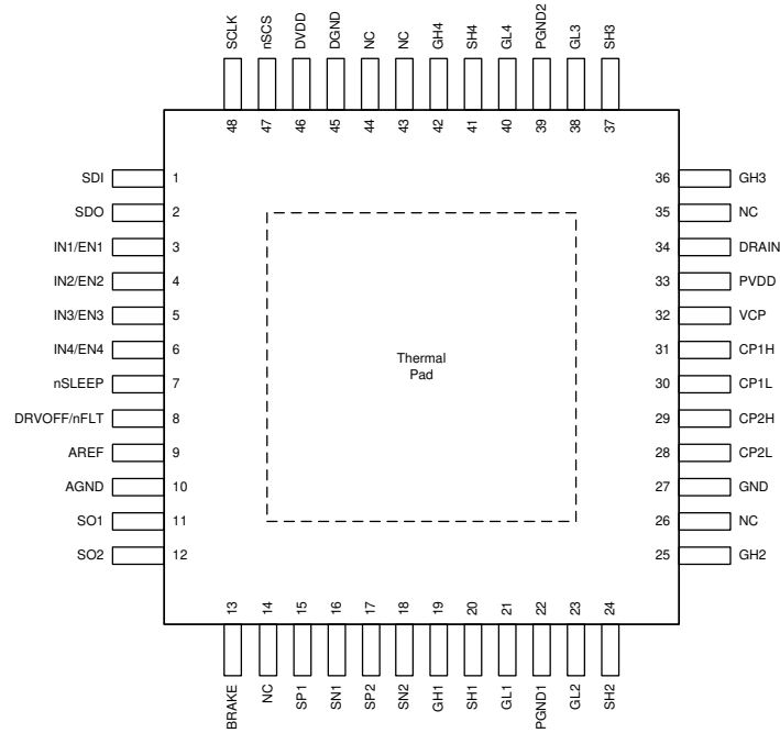
図 5-5. DRV8714S-Q1 HTQFP (PHP) 48-Pin Package Top View
