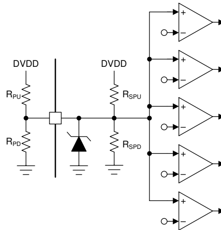
図 7-27. Six-Level Input Structure (IDRIVE, VDS)
