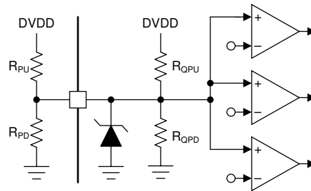
図 7-26. Quad-Level Input Structure (GAIN, MODE)
