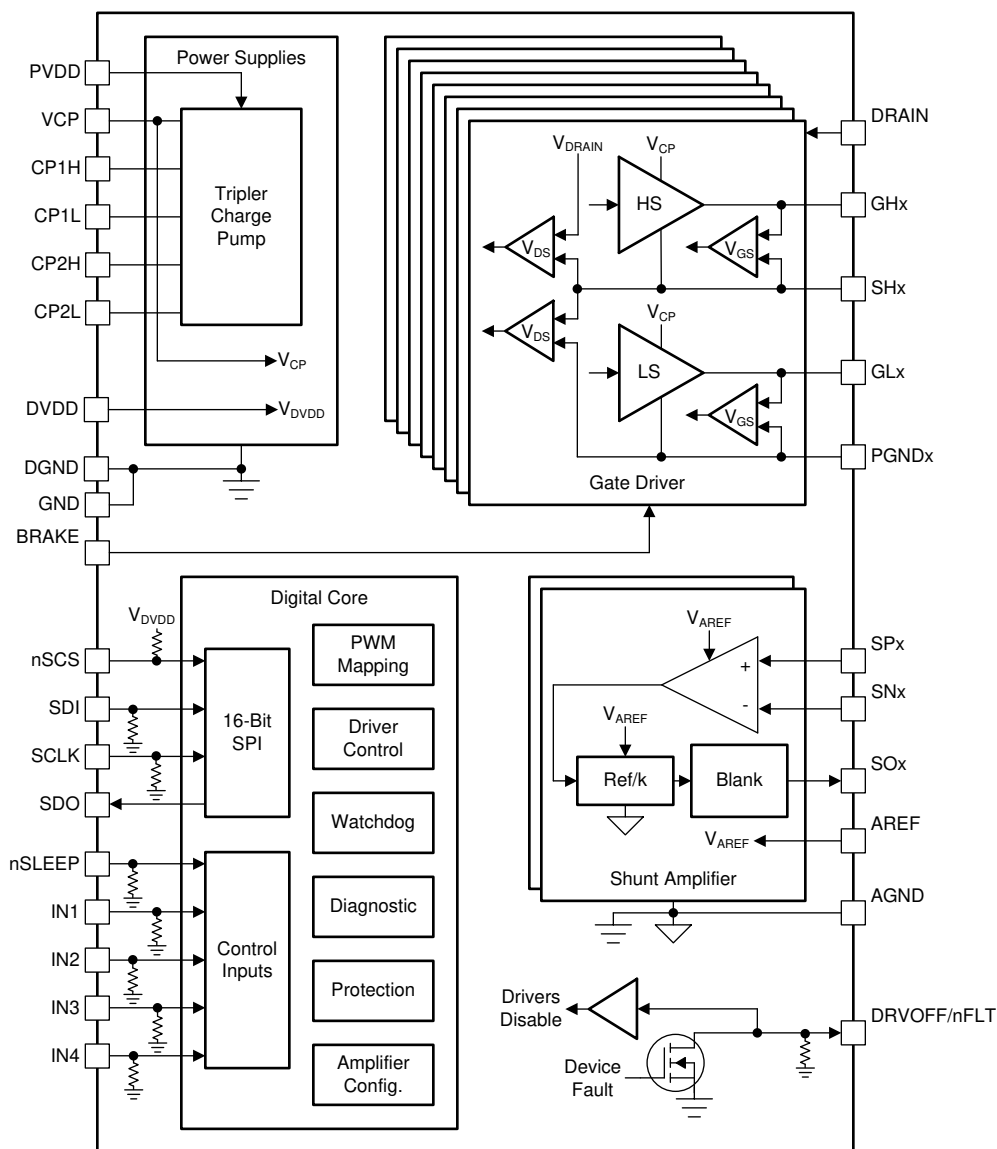
7-1. Block Diagram for DRV8718S-Q1 RVJ Package
