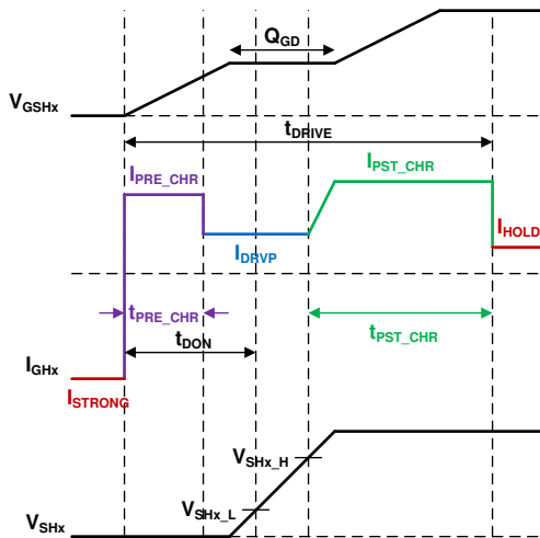
図 7-13. PDR Charge Profile
