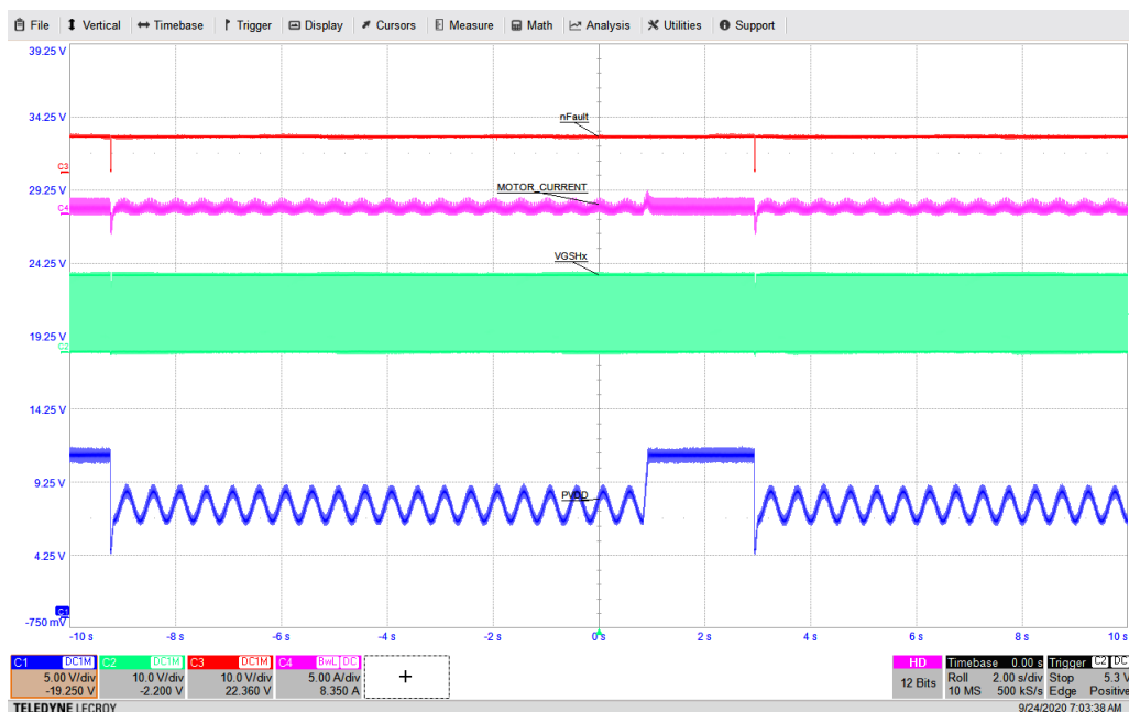
図 9-5. Driver PWM Operation During Cold Crank Pulse
