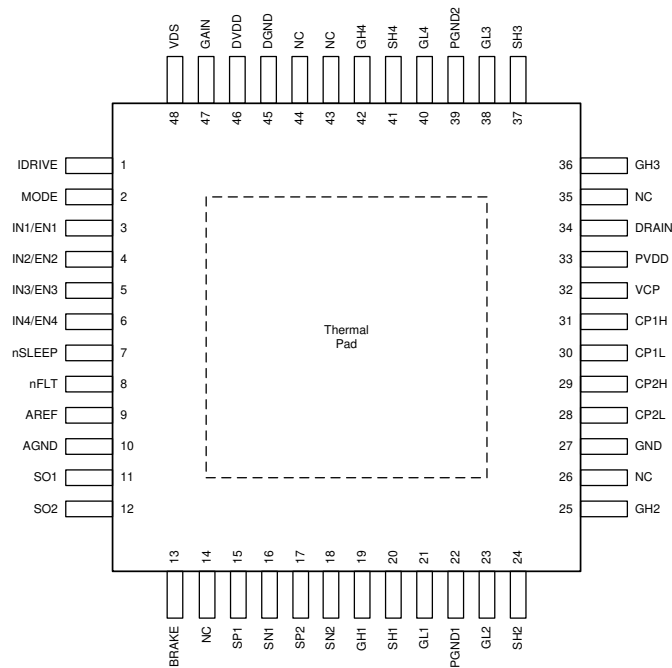
図 5-6. DRV8714H-Q1 HTQFP (PHP) 48-Pin Package Top View
