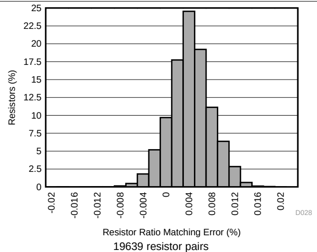
FIG 42. Resistor Pair Matching Histogram
