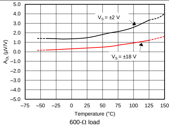
FIG 11. Open-Loop Gain vs Temperature
