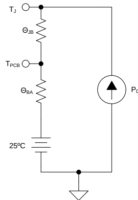
FIG 45. Approximate Thermal System Model of the INA1620 Soldered to a PCB
