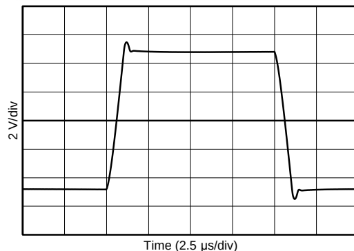
FIG 26. Large-Signal Step Response
