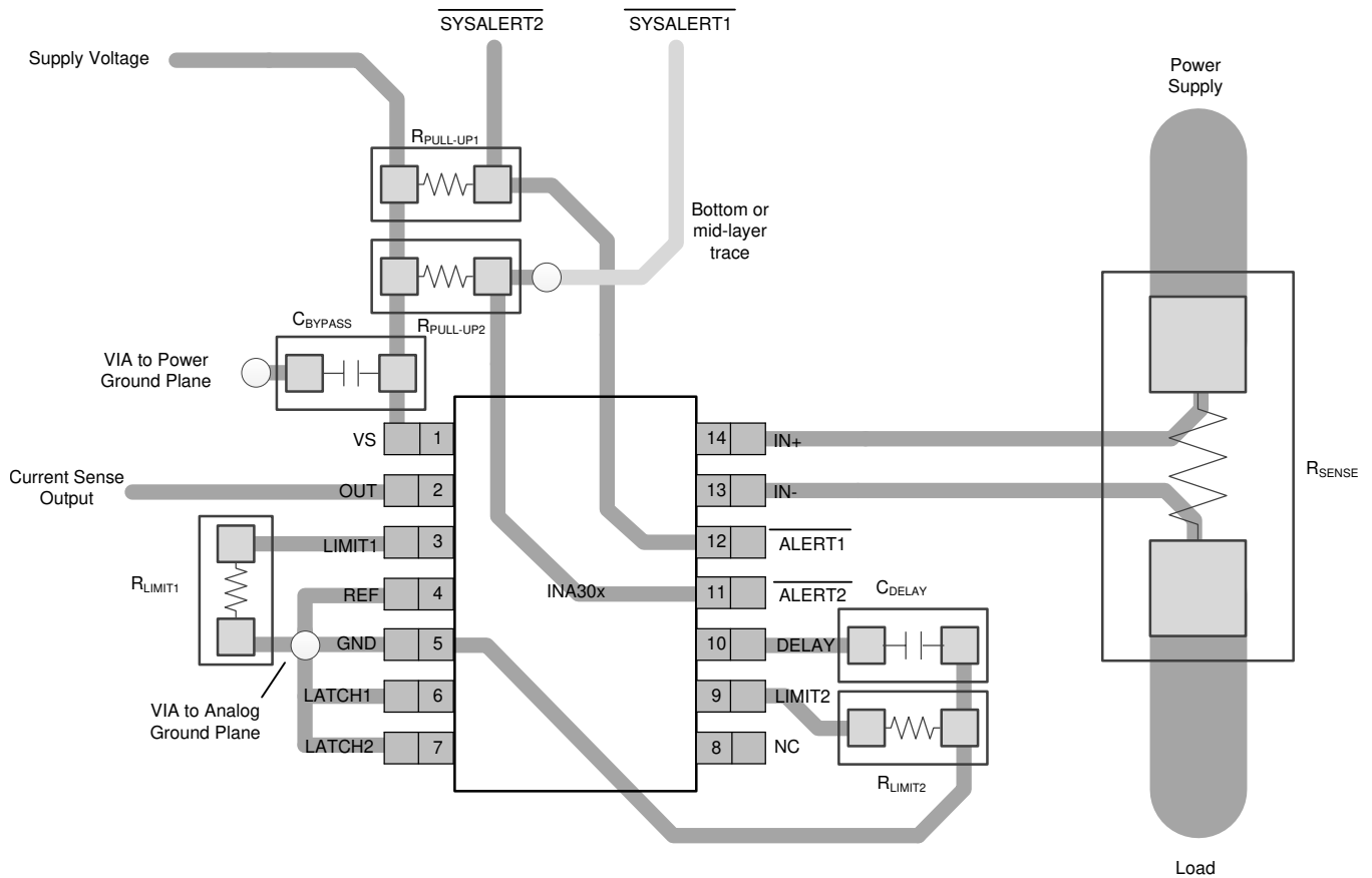
FIG 54. Recommended Layout
