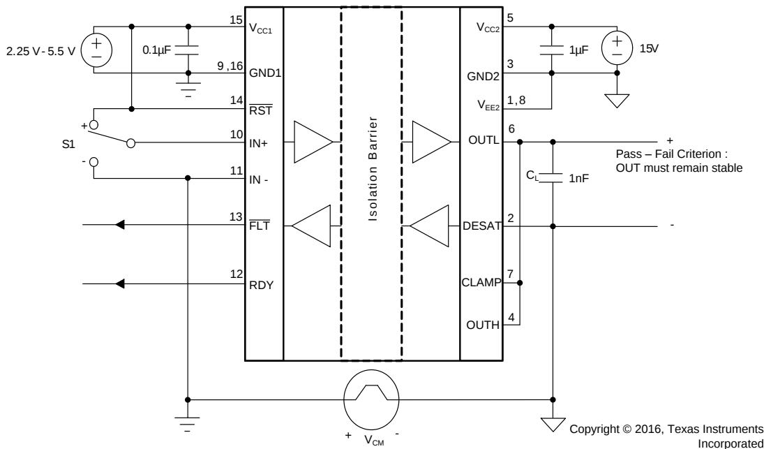
Figure 47. Common-Mode Transient Immunity Test Circuit
