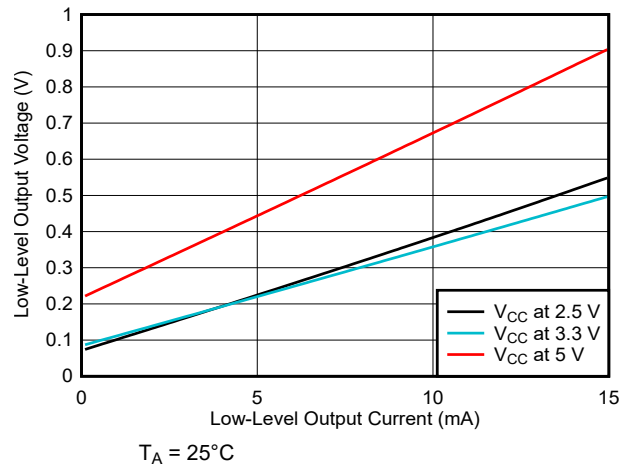
5-10. Low-Level Output Voltage vs Low-Level Output Current
