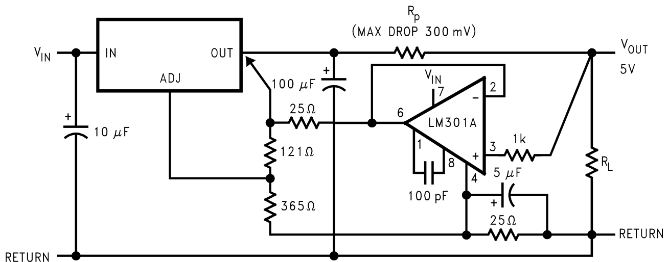
7-12. Remote Sensing
