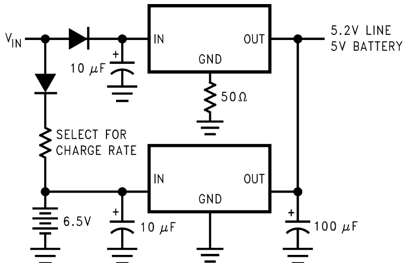
図 7-8. Battery Backup Regulated Supply
