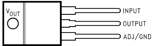
☒ 4-1. 3-Pin TO-220 Package Top View
