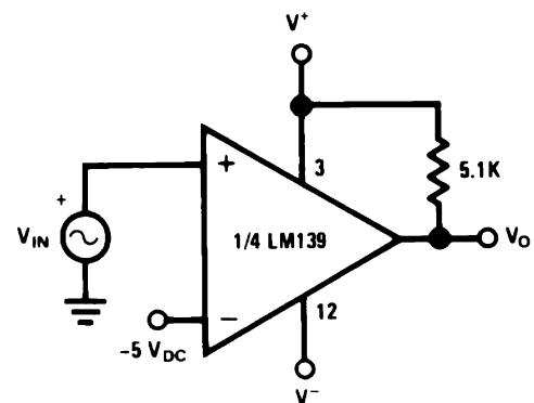
Figure 32. Comparator With a Negative Reference (V+ = +15 V DC and V- = -15 V DC )
