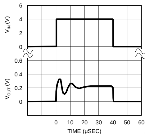
Figure 11. Start-Up Response
