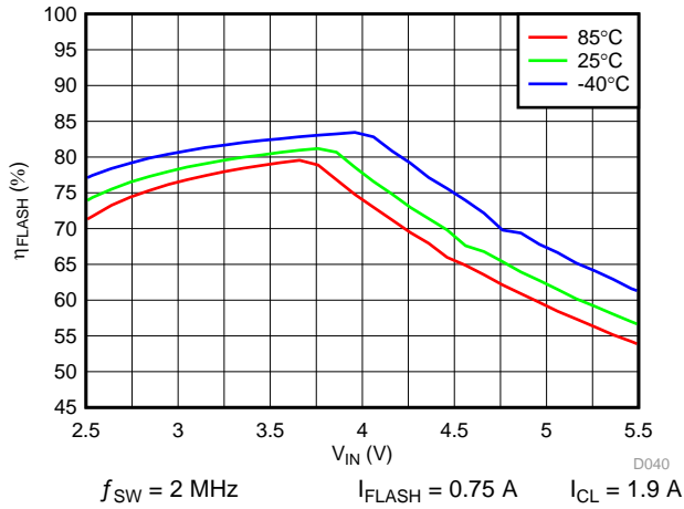
50. LED Flash Efficiency vs Input Voltage
