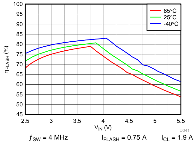
51. LED Flash Efficiency vs Input Voltage
