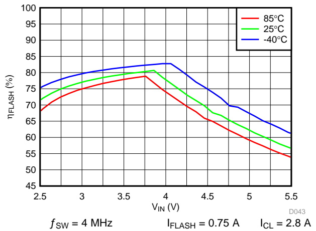
53. LED Flash Efficiency vs Input Voltage
