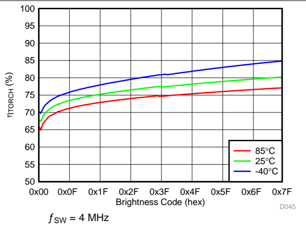
55. LED Torch Efficiency vs Brightness Code
