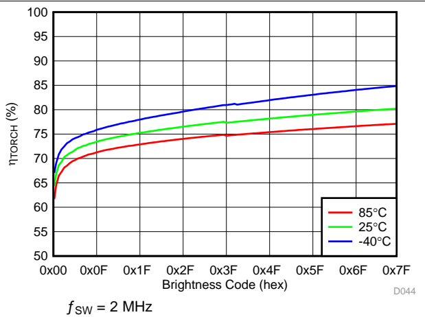
54. LED Torch Efficiency vs Brightness Code
