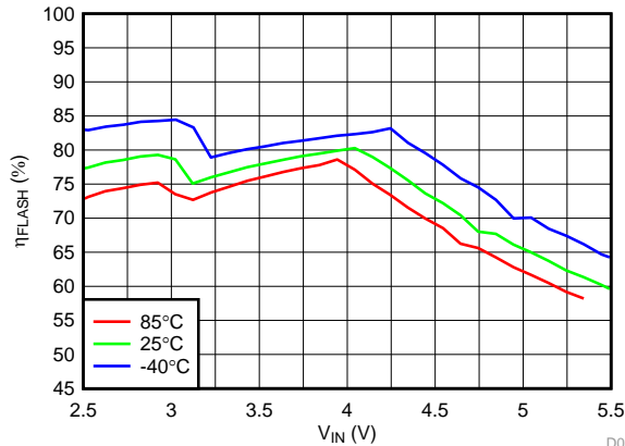
⊠ 44. LED Flash Efficiency vs Input Voltage
