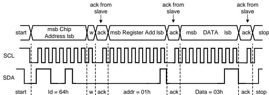
⊠ 35. Write Cycle W = Write (SDA = 0) R = Read (SDA = 1) Ack = Acknowledge (SDA Pulled Down by Either Master or Slave) ID = Chip Address, 64h for LM36010
