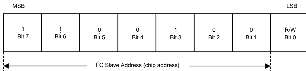
⊠ 36. I 2 C-Compatible Chip Address
