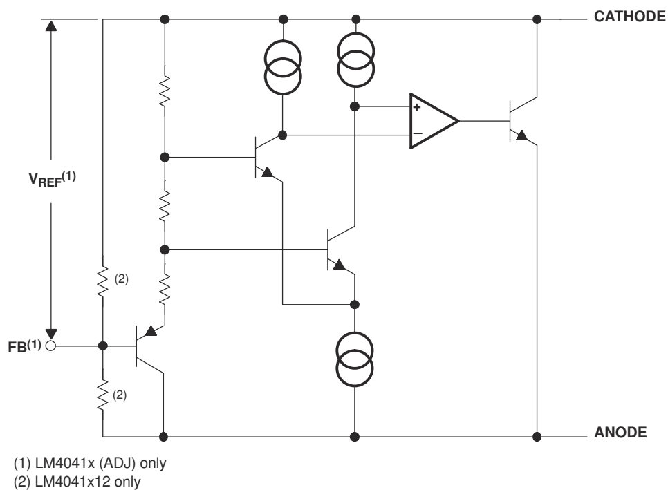
図 6-1. Functional Block Diagram
