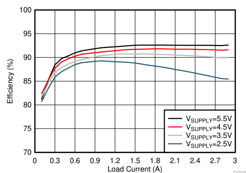
効率 ( V_{LOAD} = 6.8V , F_{SW} = 440kHz )
