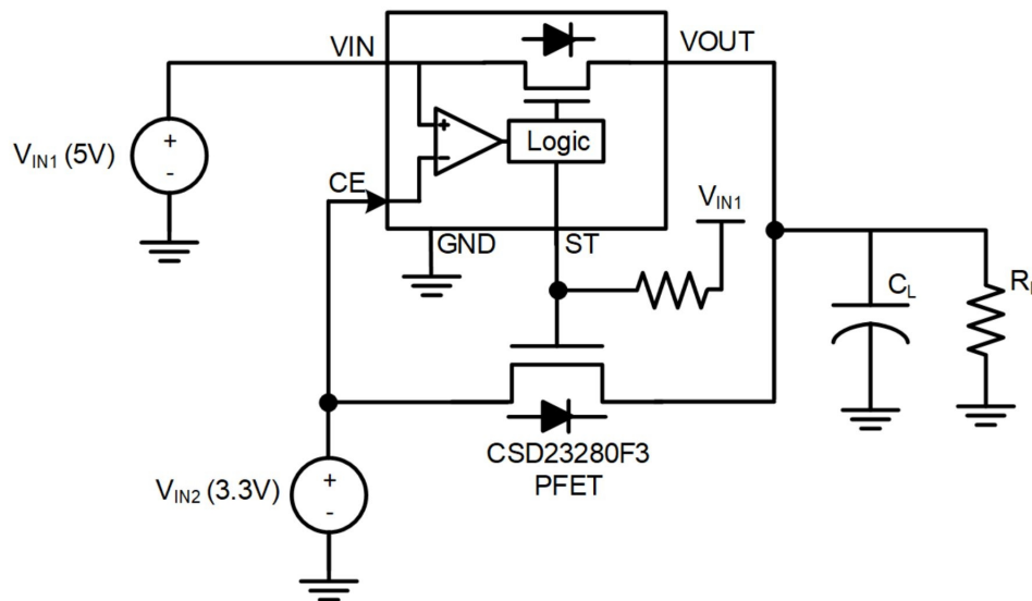
✎ 20. ORing with a Discrete MOSFET
