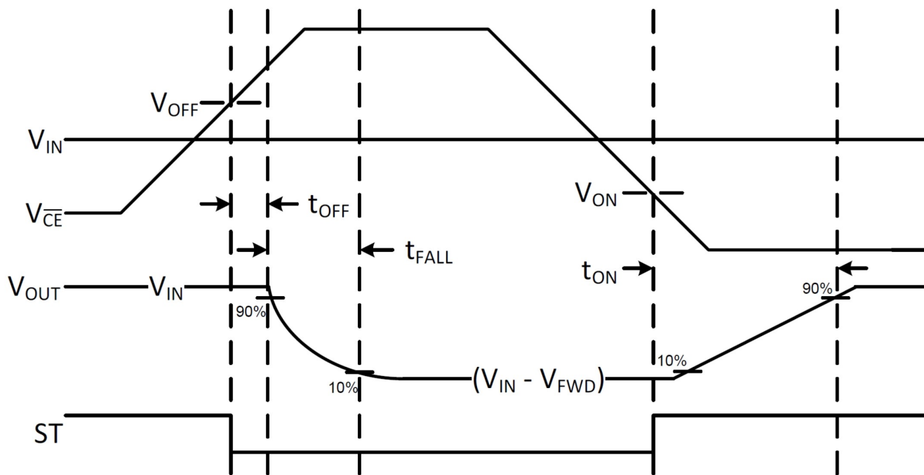
Figure 11. Timing Diagram
