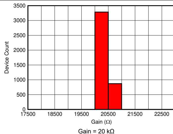
6-46. Transimpedance Gain (High) Distribution
