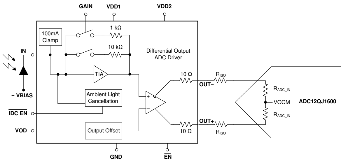
8-2. LMH32401 to ADC Interface with a Matching Resistor Network
