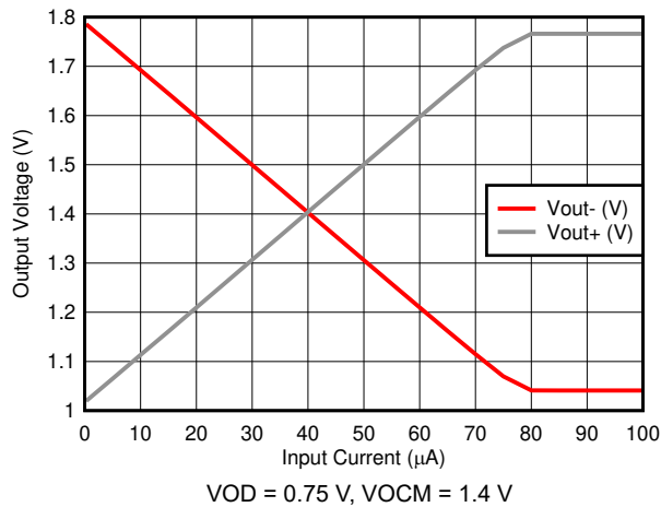
6-39. High-side Swing vs Input Current
