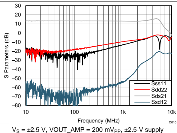
Figure 10. S-Parameters Single-Ended Input
