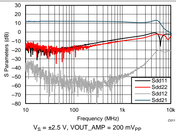
Figure 11. S-Parameters Differential Input ( \pm 2.5\text{-V} Supply)
