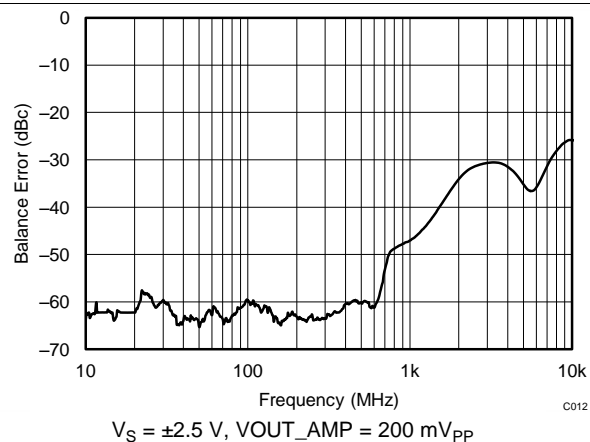
Figure 12. Balance Error
