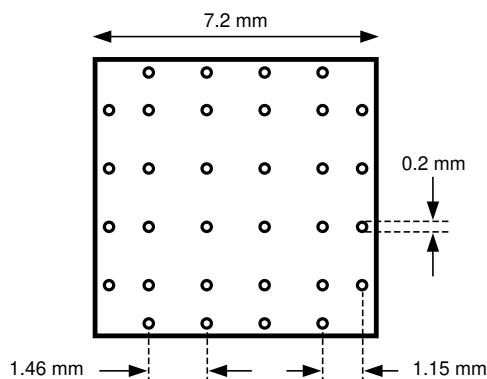
☒ 8-14. Recommended Land and Via Pattern
