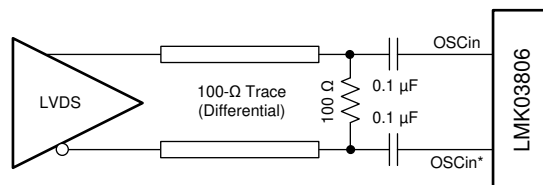
8-4. OSCin/OSCin* Termination for an LVDS Reference Clock Source
