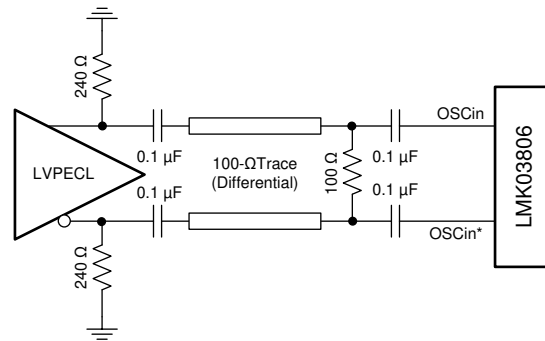
図 8-5. OSCin/OSCin* Termination for an LVPECL Reference Clock Source
