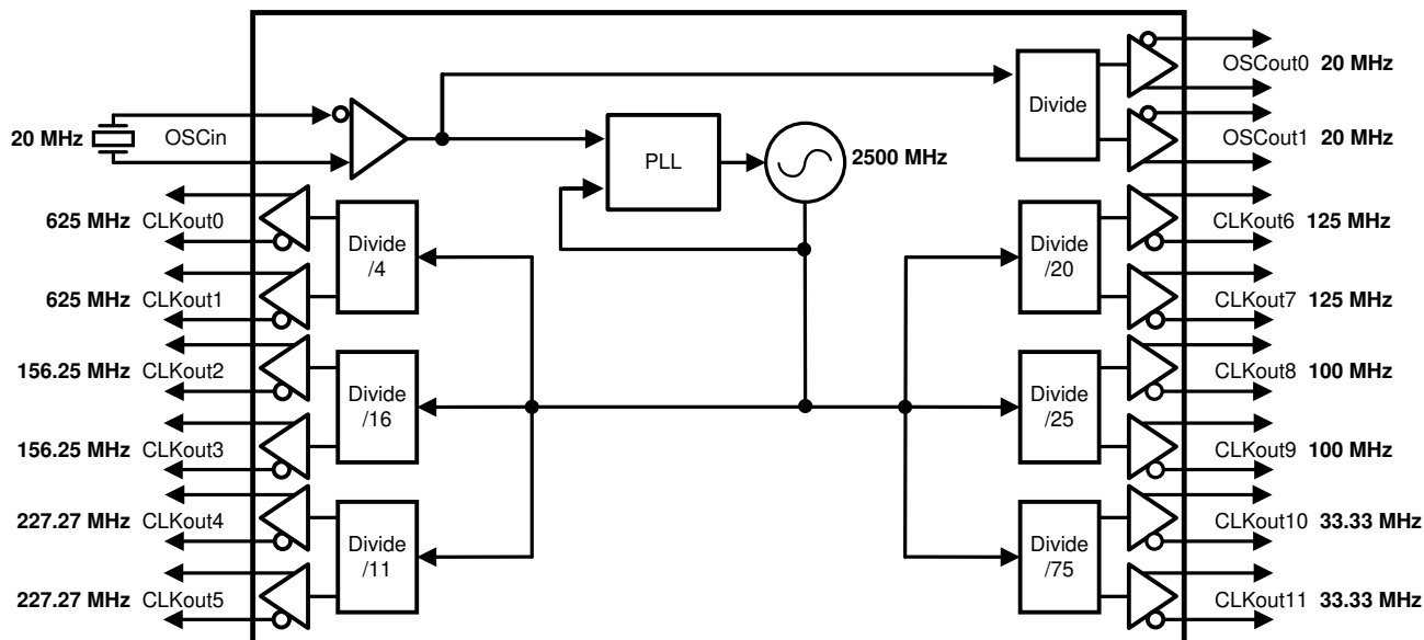
図 7-2. 10-Gigabit Ethernet Reference Clocks
