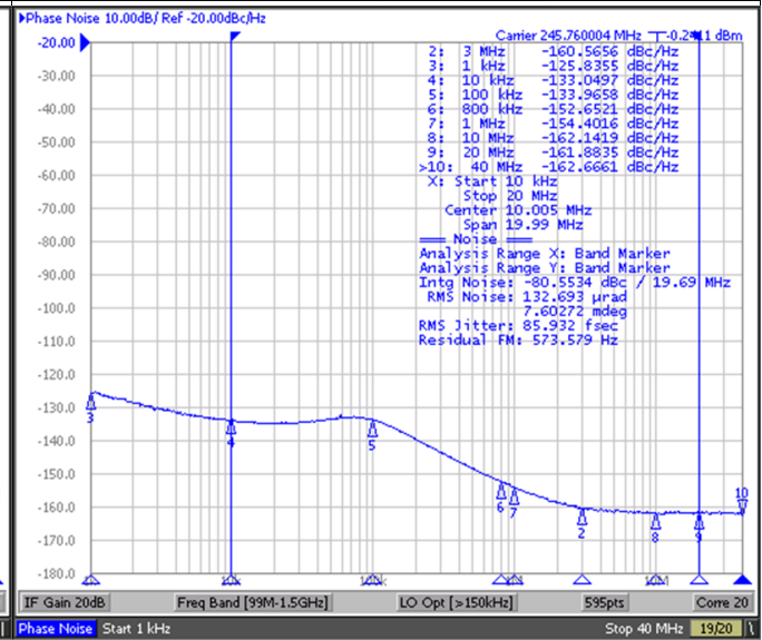
Figure 3. LMK04821 DCLKout2 Phase Noise
