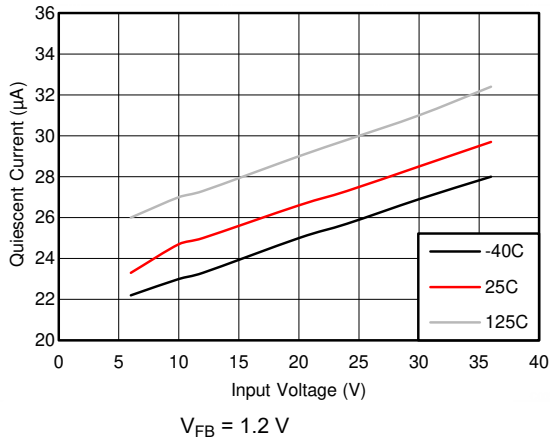
7-1. Non-Switching Input Supply Current
