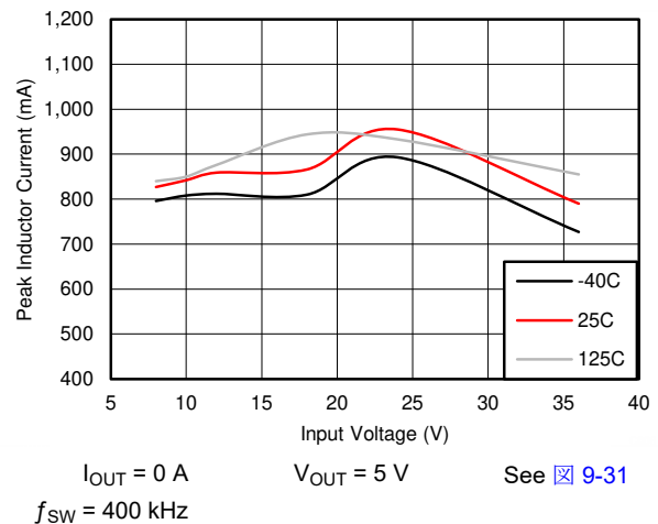
7-6. I_{PEAK-MIN}
