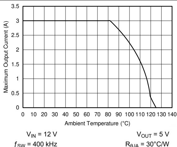
Figure 9-5. Maximum Output Current versus Ambient Temperature
