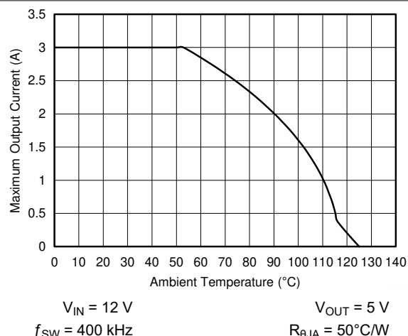
Figure 9-6. Maximum Output Current versus Ambient Temperature
