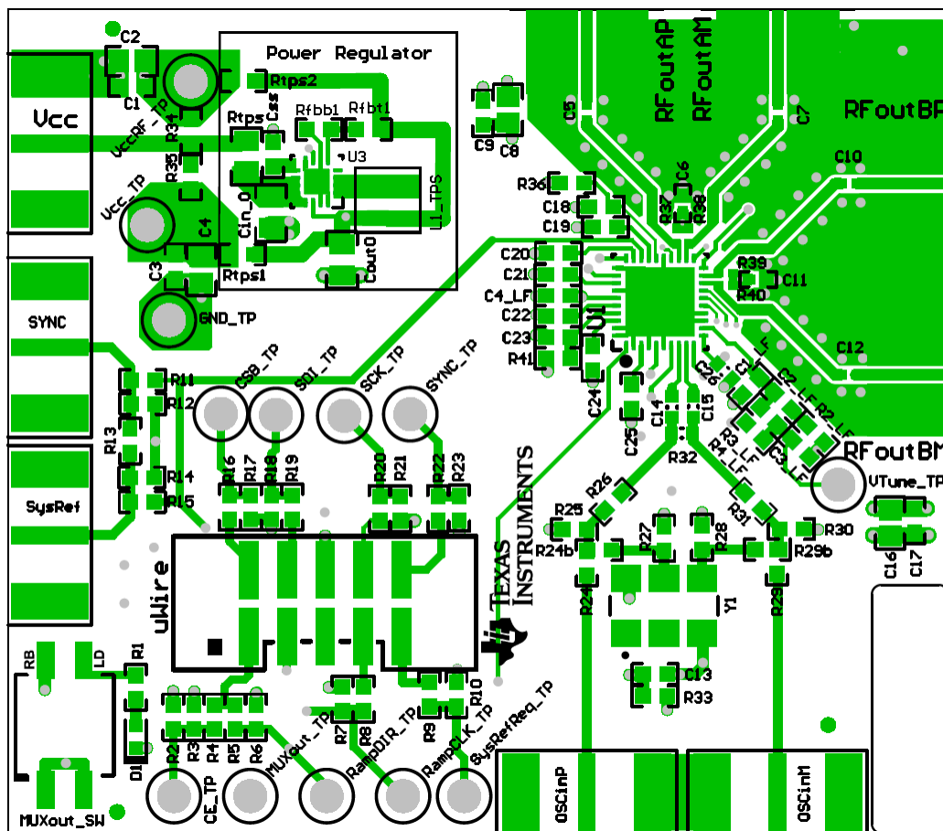
189. Layout Example
