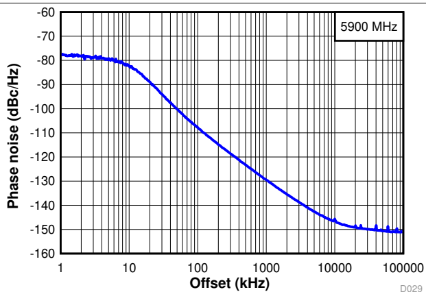
FIG 20. Narrow Band Phase Noise at 5.9 GHz
