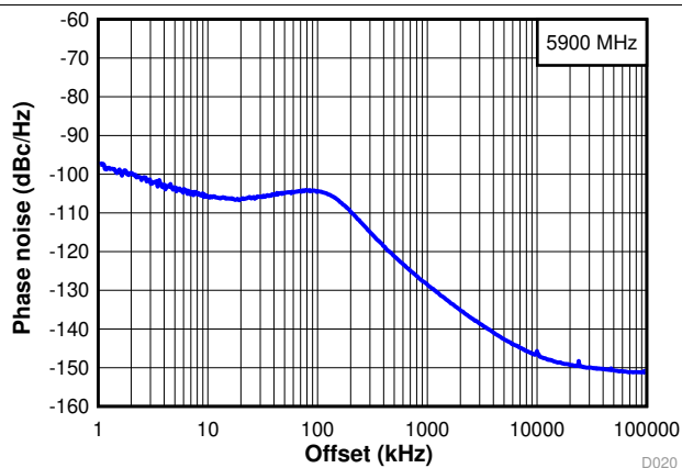
FIG 19. Wide Band Phase Noise at 5.9 GHz
