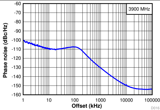
FIG 11. Wide Band Phase Noise at 3.9 GHz
