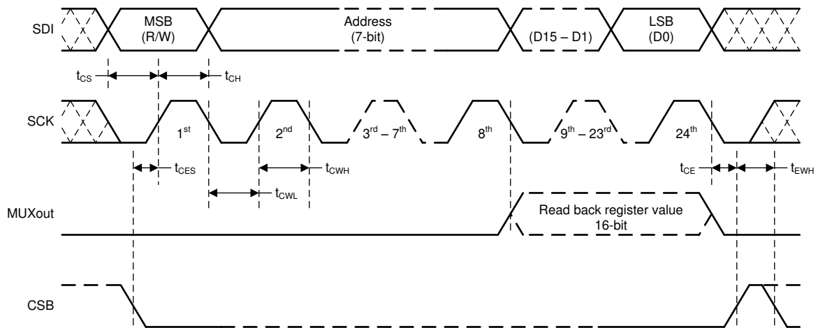
✎ 1. Serial Interface Timing Diagram
