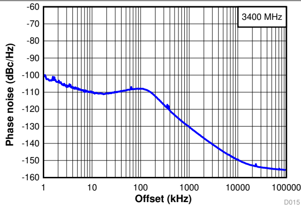
FIG 9. Wide Band Phase Noise at 3.4 GHz
