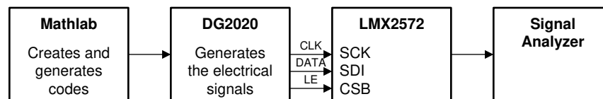
✎ 182. Application Example Test Setup
