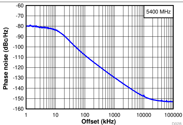
FIG 18. Narrow Band Phase Noise at 5.4 GHz
