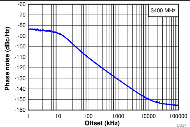
FIG 10. Narrow Band Phase Noise at 3.4 GHz
