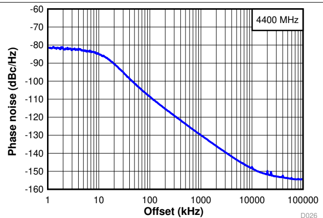
FIG 14. Narrow Band Phase Noise at 4.4 GHz
