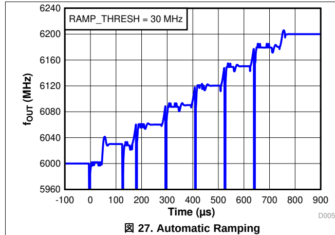
Figure 27. Automatic Ramping
