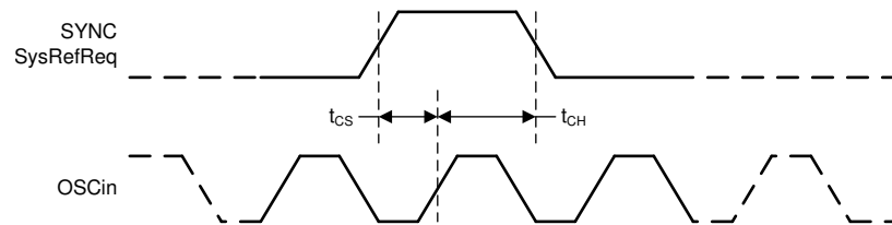
✎ 2. Trigger Signals Timing Diagram
