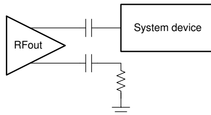
FIG 169. Unused Output Buffer Differential Pin
