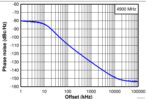
FIG 16. Narrow Band Phase Noise at 4.9 GHz
