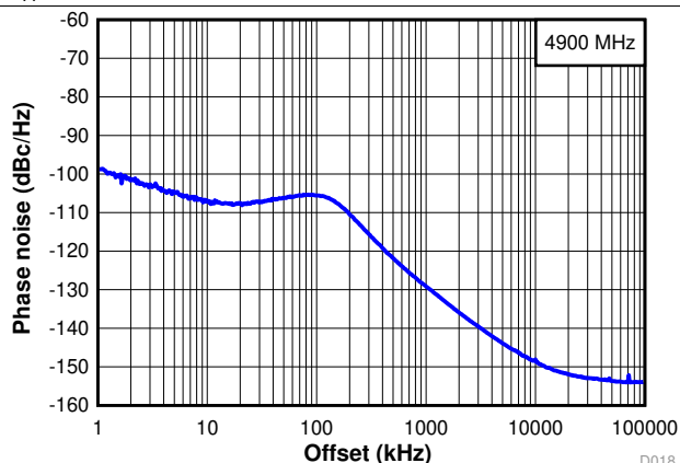
FIG 15. Wide Band Phase Noise at 4.9 GHz
