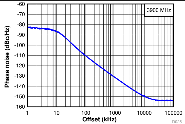
FIG 12. Narrow Band Phase Noise at 3.9 GHz
