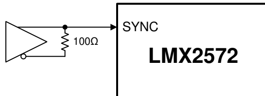
図 171. Driving SYNC Pin With Differential Signal
