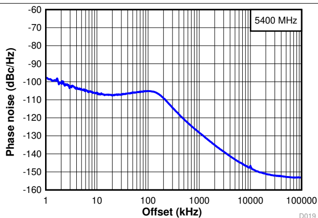
FIG 17. Wide Band Phase Noise at 5.4 GHz
