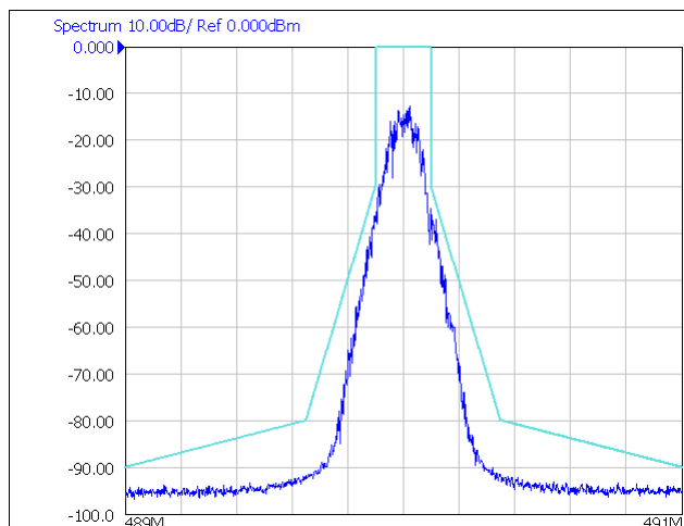
✎ 183. Gaussian 4FSK Modulated Spectrum
