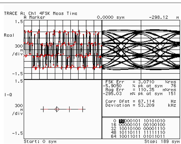
✎ 184. Gaussian 4FSK Modulation Quality
