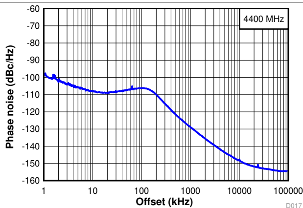
FIG 13. Wide Band Phase Noise at 4.4 GHz
