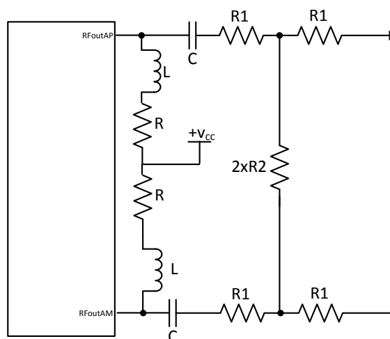
75. Termination of Unused Output
