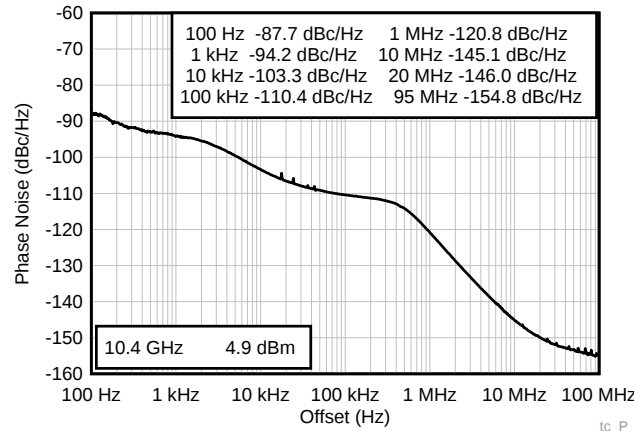
FIG 78. Results for Loop Filter Design
