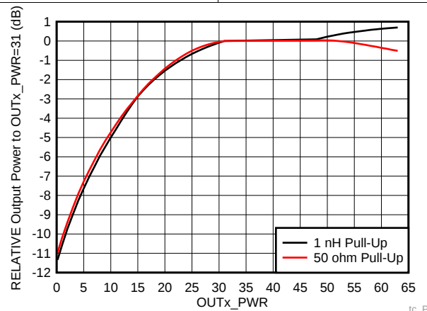
FIG 16. Output Power vs Pull-up
