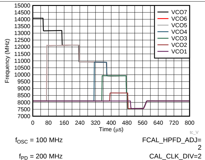
FIG 20. Impact of VCO_SEL on VCO Calibration Time
