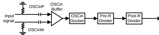
FIG 22. Reference Path Diagram
