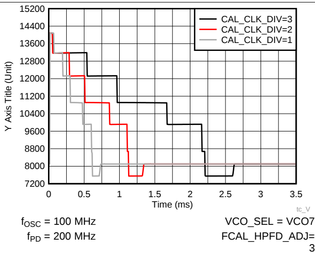
FIG 19. Impact of CAL_CLK_DIV on VCO Calibration Time
