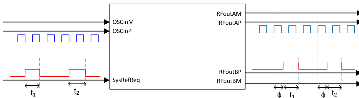
FIG 29. SYSREF Out In Repeater Mode
