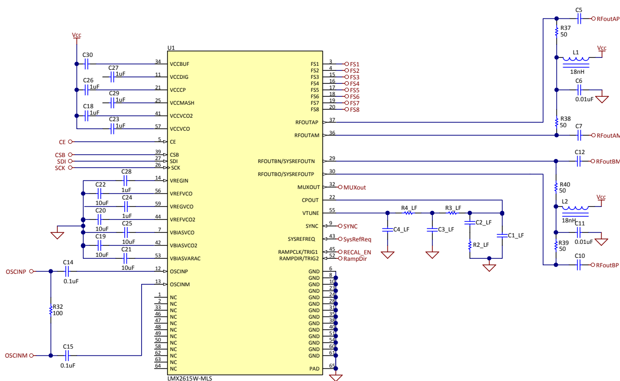
76. Typical Application Schematic
