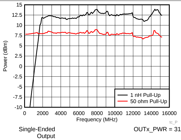
FIG 16. Output Power vs Pull-up
