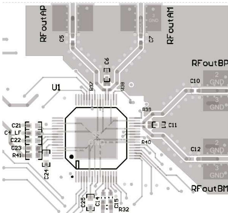
FIG 79. LMX2615 Layout Example
