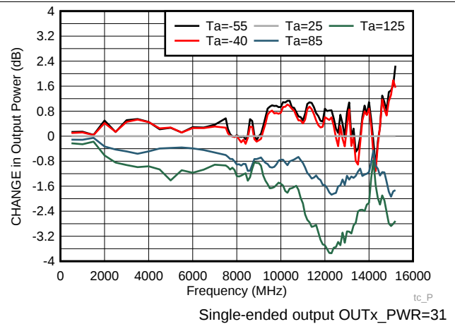
FIG 17. CHANGE in Output Power vs Temperature
