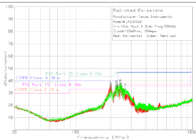
Figure 32. Radiated Emissions 12-V Input, 3.3-V Output, 20-A Load (EN55022 Class A)
