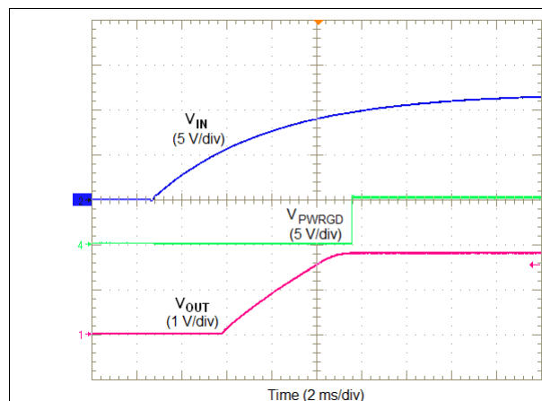
Figure 18. Start-Up Waveforms
