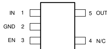
図 4-3. DBV Package, 5-Pin SOT-23 (Top View)
