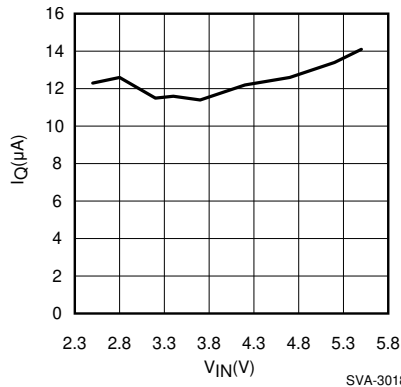
図 5-1. Quiescent Current vs Input Voltage
