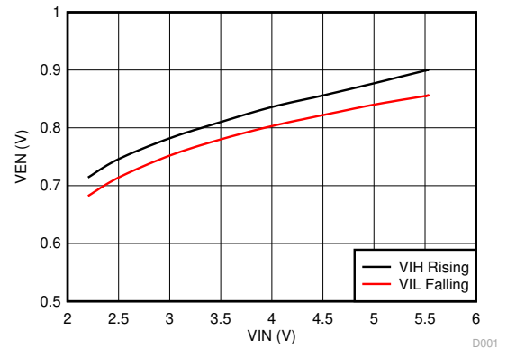
図 5-2. V_{EN} Thresholds vs V_{IN}
