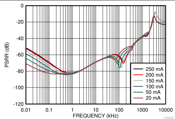
5-20. PSRR Loads Averaged 10Hz to 10MHz
