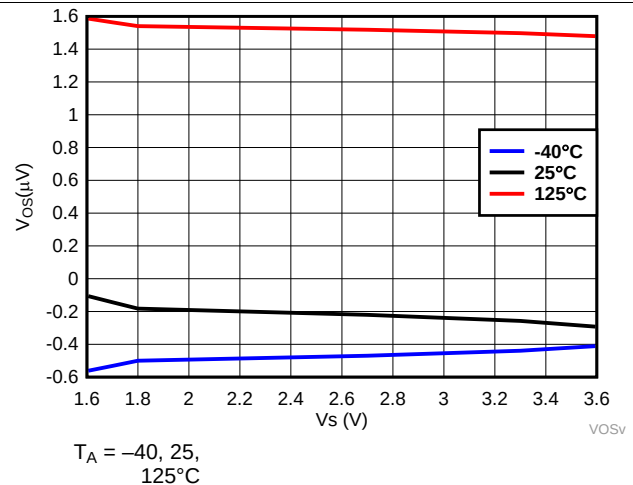
FIG 10. Offset Voltage vs Supply Voltage
