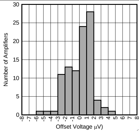
FIG. 1. Offset Voltage Distribution, V_S = 1.8\text{ V}
