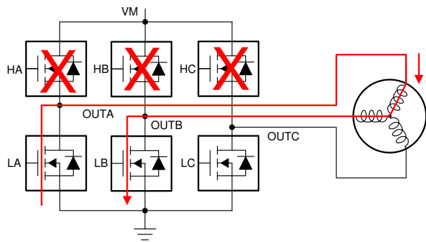
Figure 8-36. Brake State
