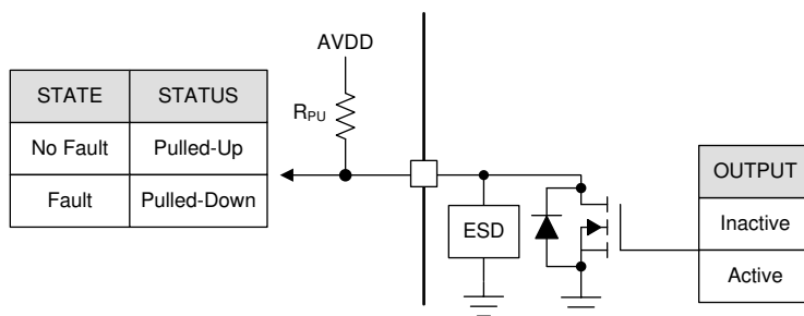
8-25. Open Drain
