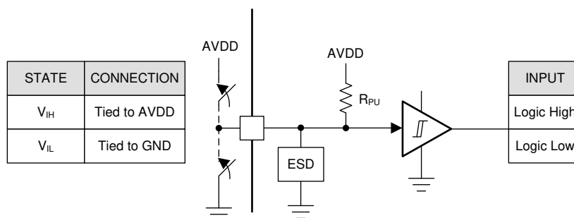
Figure 8-24. Logic nSCC
