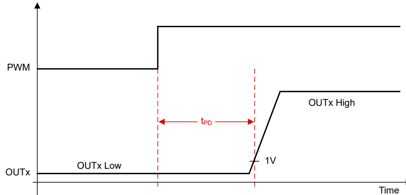
FIG 8-20. Propagation Delay Timing
