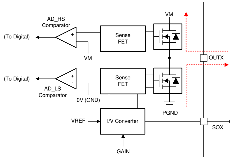
图 8-29. Active Demagnetization Operation
