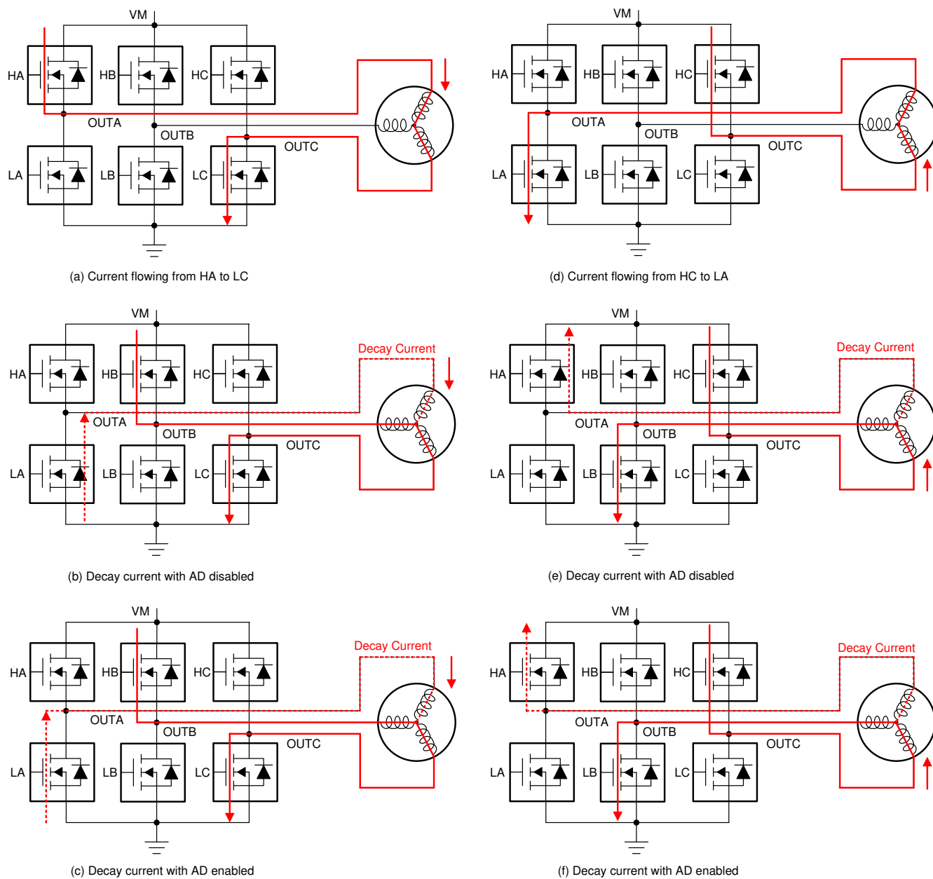
8-30. ASR in BLDC Motor Commutation
