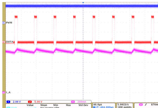
9-16. Driver 100% Operation with Current Chopping
