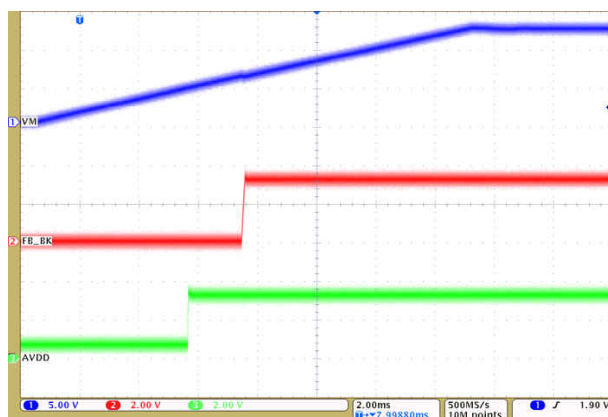
Figure 9-13. Power Management
