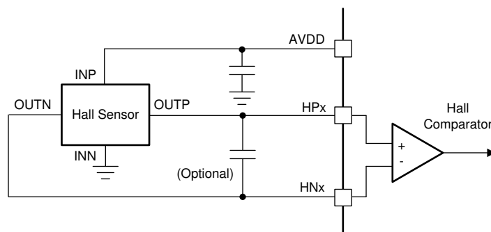
FIG 9-3. Typical Hall Sensor Configuration
