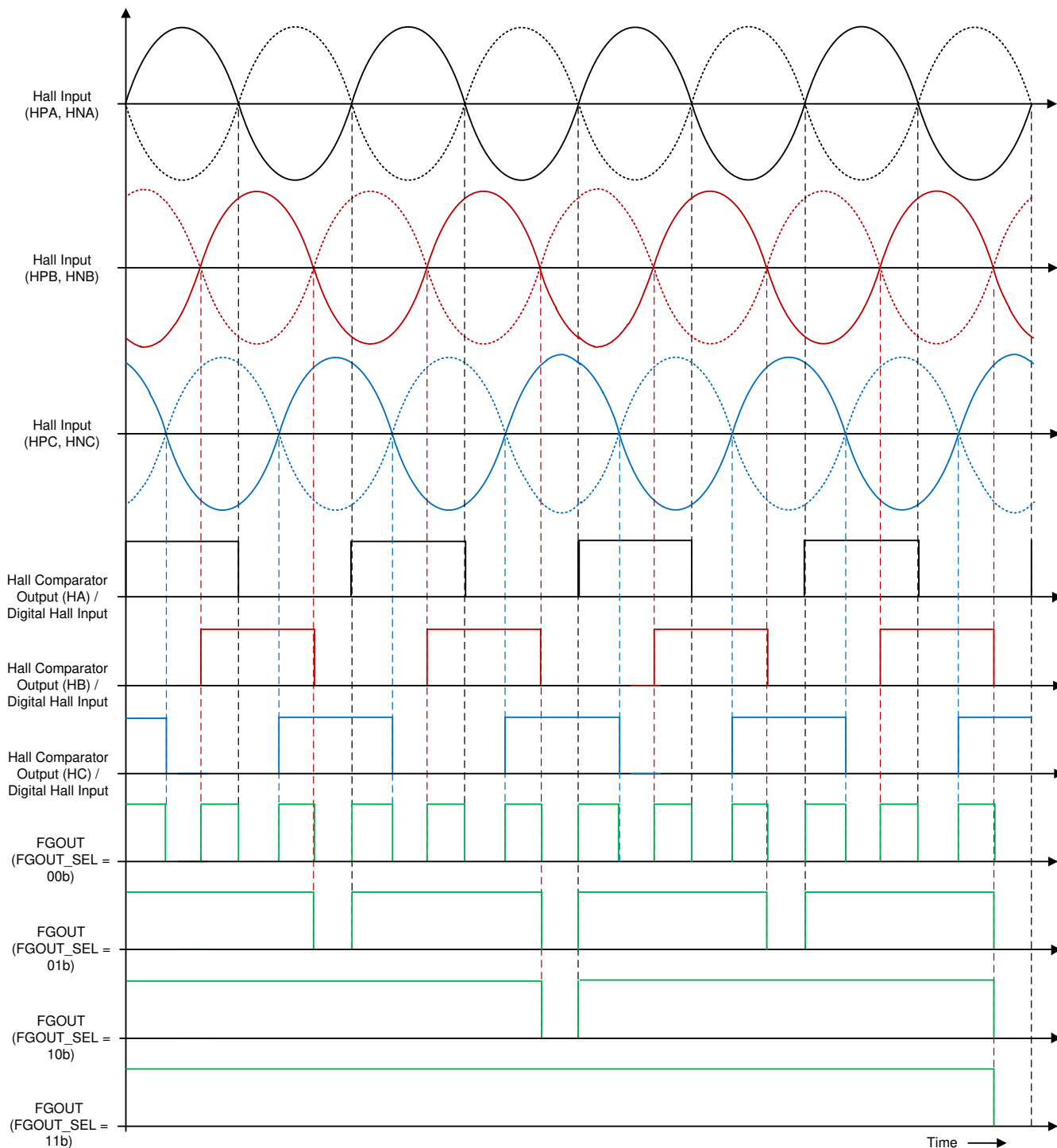
8-41. FGOUT Signal
