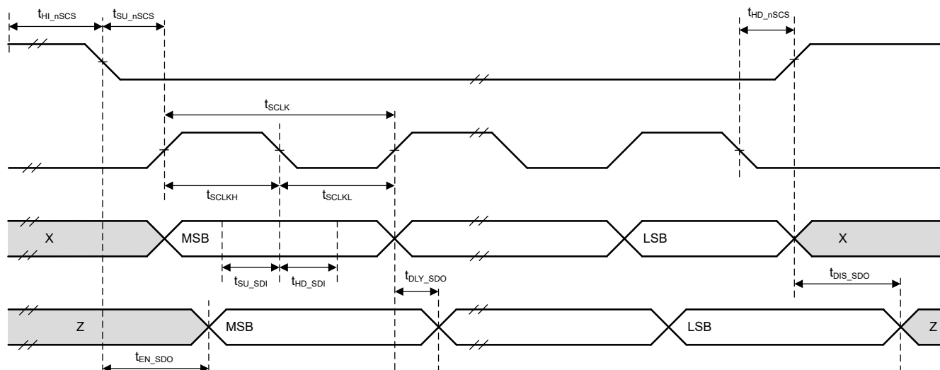
Figure 7-1. SPI Secondary Mode Timing Diagram
