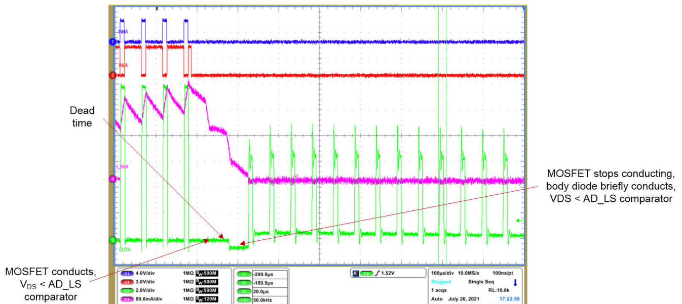
9-8. Active demagnetization enabled in MCT8316Z
