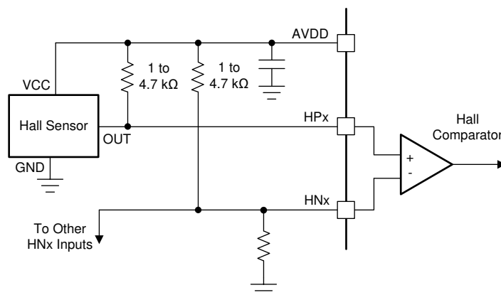
FIG 9-4. Open-Drain Hall Sensor Configuration
