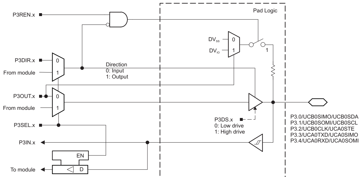
☒ 6-4. Port P3 (P3.0 to P3.4) Diagram
