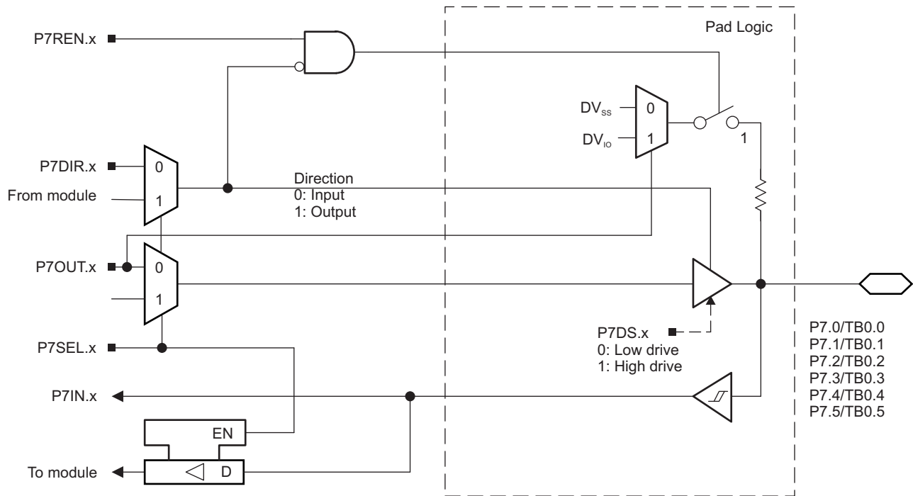
❏ 6-12. Port P7 (P7.0 to P7.5) Diagram
