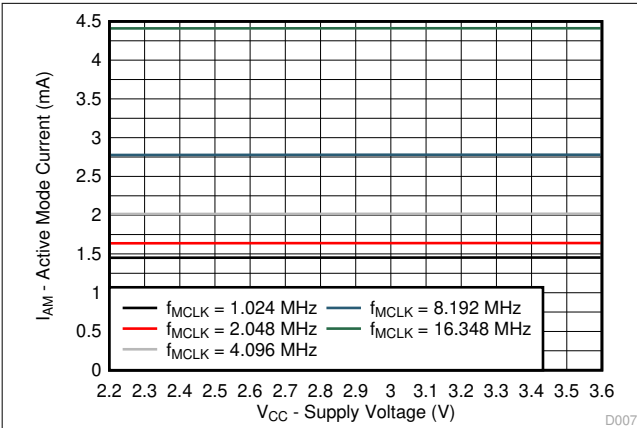
8-2. Active Mode Current vs Supply Voltage
