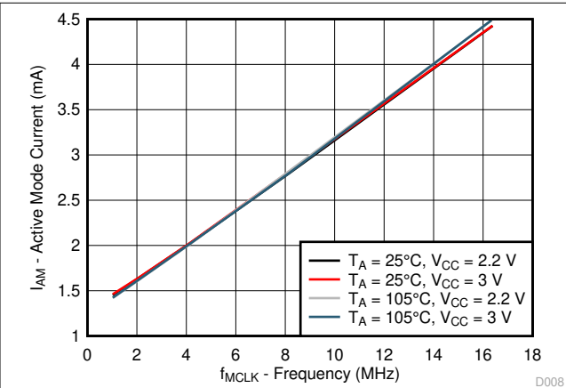
8-3. Active Mode Current vs MCLK Frequency
