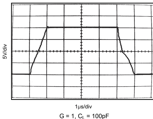
FIG 5-21. Large-Signal Step Response
