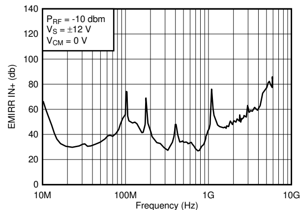
Figure 46. OPA211 EMIRR
