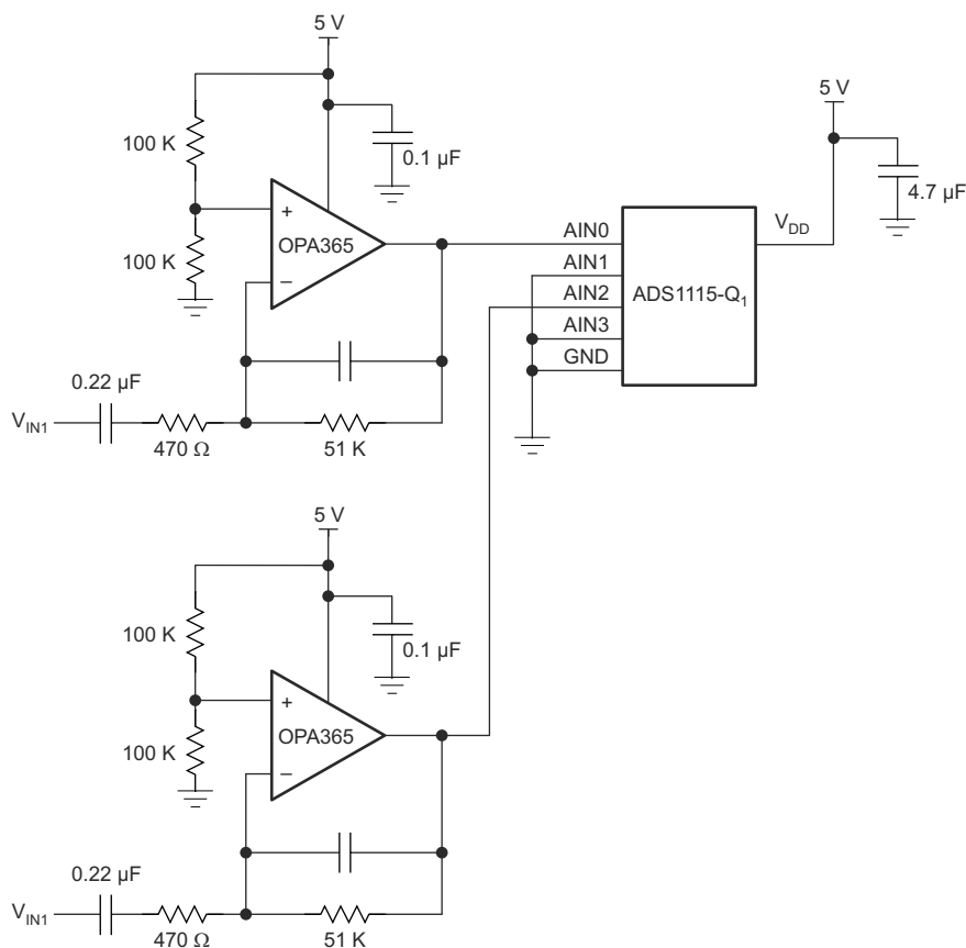
FIG 8-6. Driving the ADS1115-Q1
