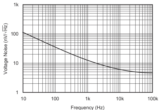
6-14. Input Voltage Noise Spectral Density
