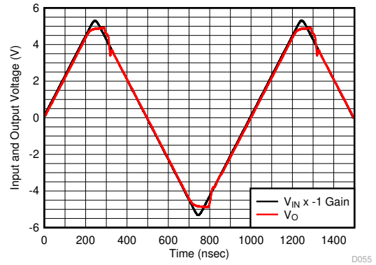
7-14. Output Overdrive Recovery
