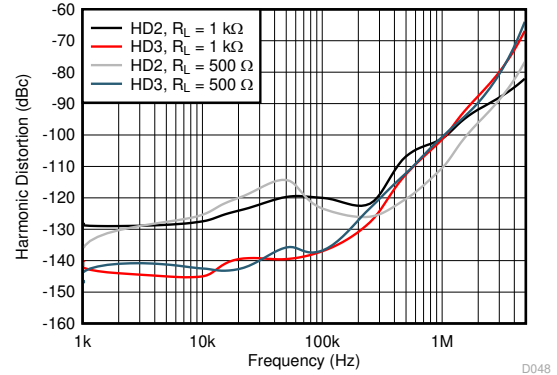
See 9-1 , gain = 2 V/V
