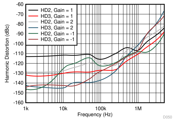
See 9-1 and 9-2 , R_F = 0 \Omega
