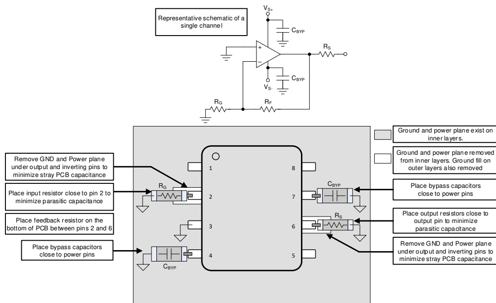
11-1. Layout Recommendation
