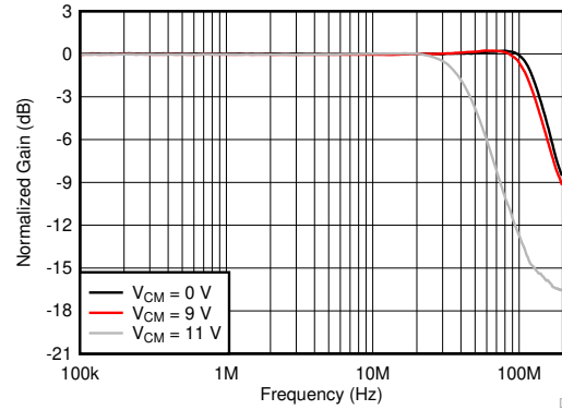
7-19. Small-Signal Frequency Response vs Output Common-Mode Voltage
