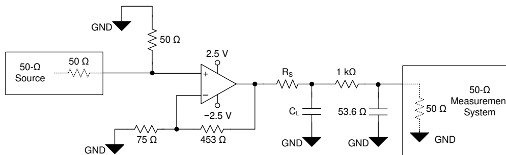
Figure 8-3. Capacitive Load Driver Configuration
