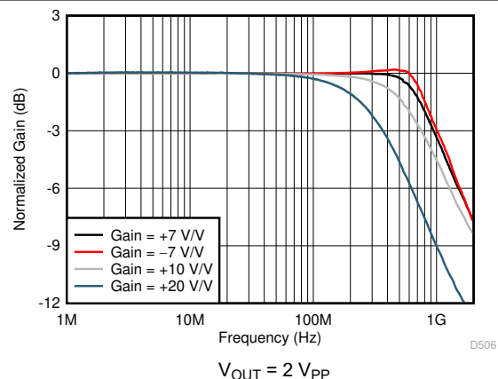
Figure 7-6. Large-Signal Frequency Response vs Gain
