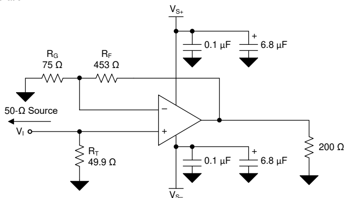
FIG 10-11. Split and Single Supply Circuit Configuration
