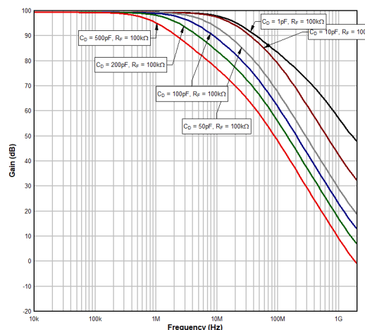
FIG 10-10. 3 Photodetector Input Characteristics TIA Frequency Response
