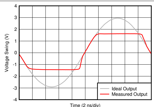
Figure 7-20. Large-Signal Transient Response
