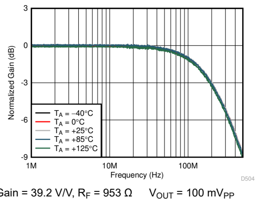
Figure 7-4. Small-Signal Frequency Response vs Ambient Temperature
