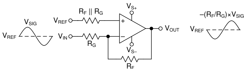
Figure 9-2. Inverting Amplifier
