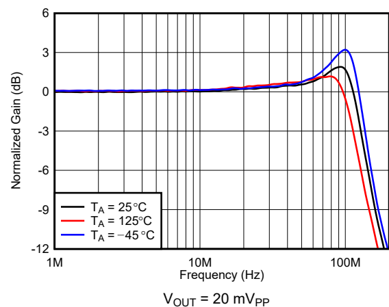
7-5. Frequency Response vs Ambient Temperature
