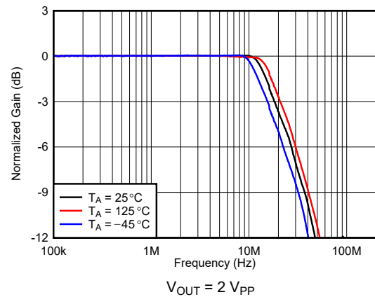
7-8. Frequency Response vs Ambient Temperature
