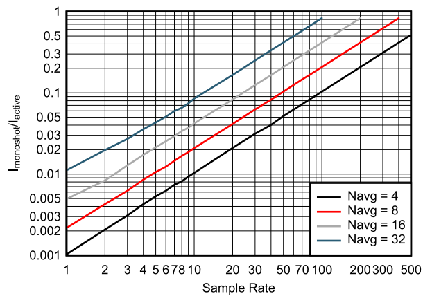
図 8. AVDD3 Supply Current in Monoshot Mode
