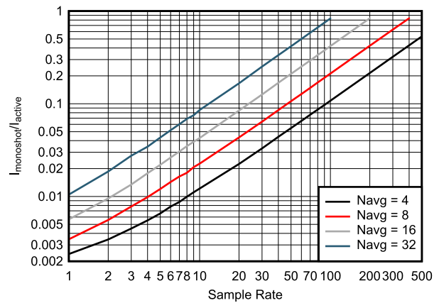
図 9. IOVDD Supply Current in Monoshot Mode
