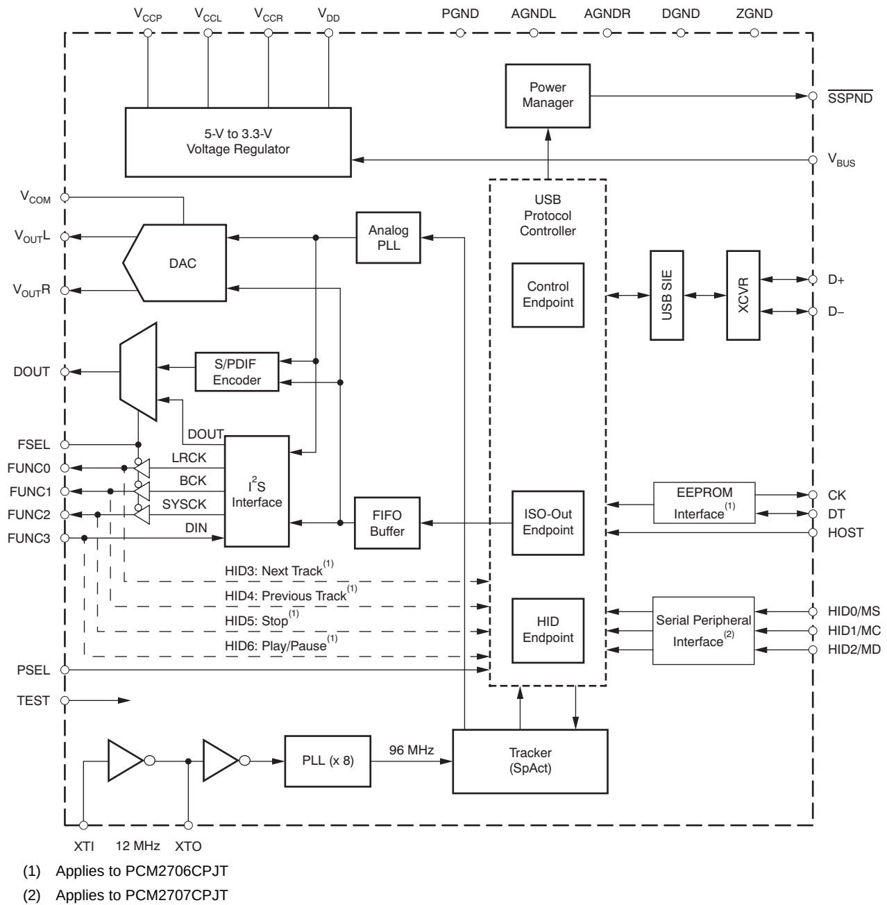
Figure 27. PCM2706C/PCM2707C
