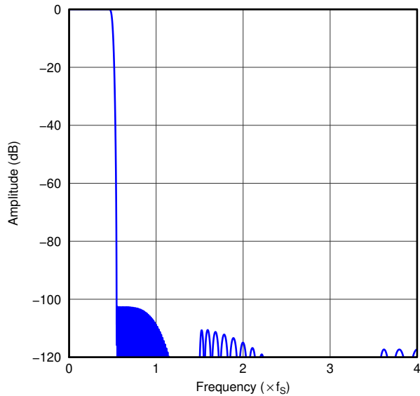
Figure 46. High-Attenuation x8 Interpolation Filter Frequency Response, Single Rate
