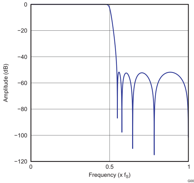
Figure 39. Low latency x2 Interpolation Filter Frequency Response
