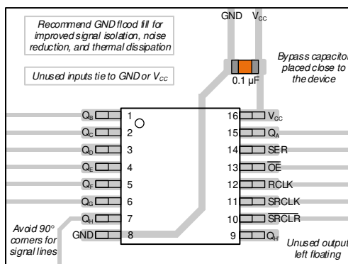
FIG 11-1. Example layout for the SN74HCS595.
