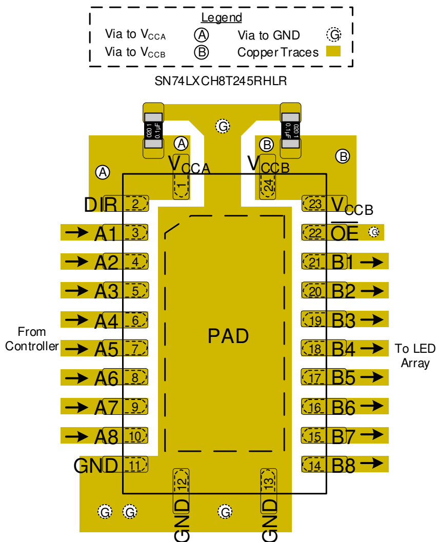
11-1. Layout Example
