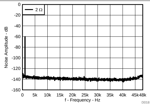
20. Noise vs Frequency
