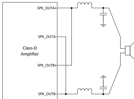
Figure 39. Pre-Filter PBTTL
