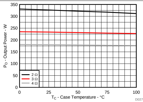
19. Output Power vs Temperature
