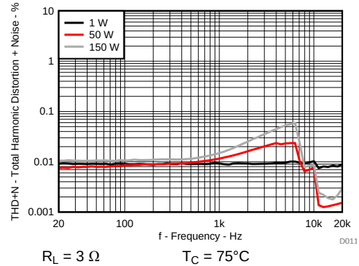
FIG 14. Total Harmonic Distortion+Noise vs Frequency
