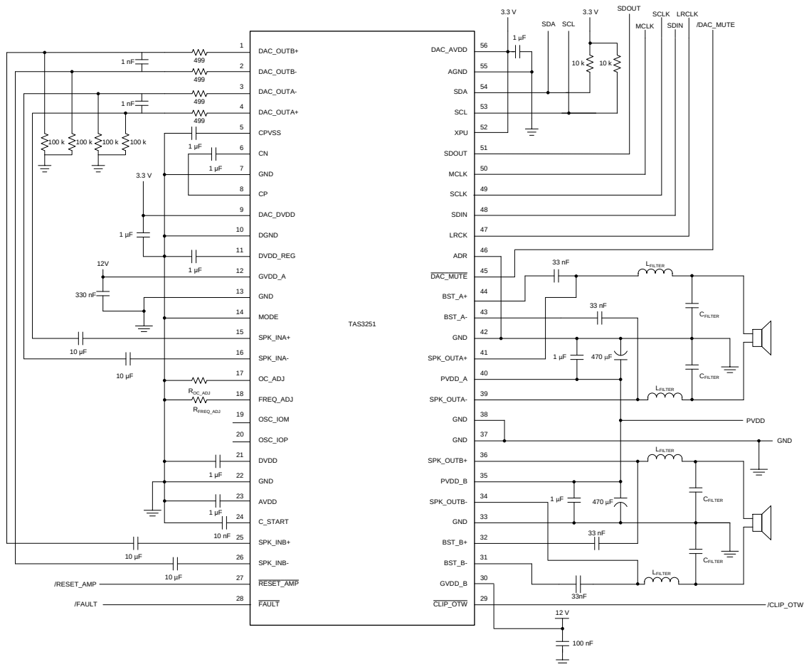
FIG 122. Bridge-Tied Load (BTL) Application Diagram
