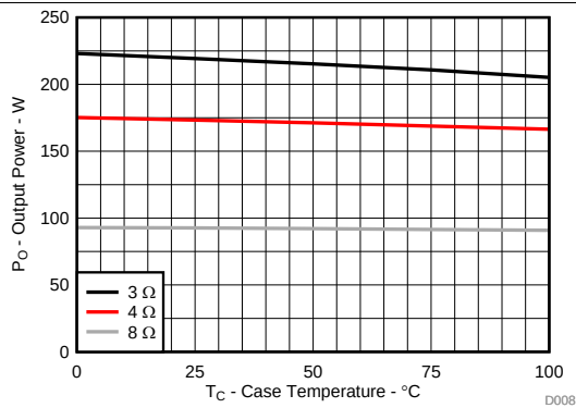
⊠ 11. Output Power vs Temperature
