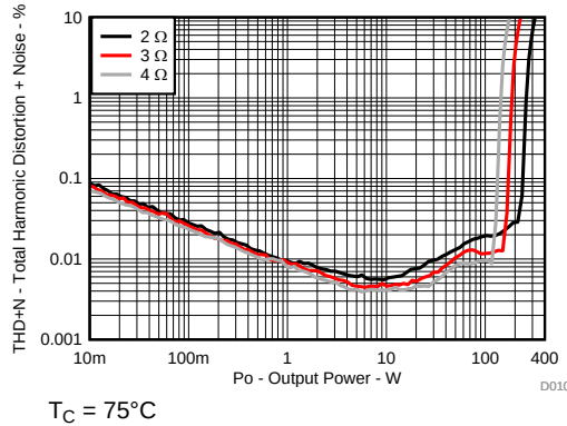
FIG 13. Total Harmonic Distortion+Noise vs Output Power
