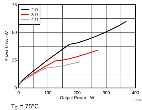
FIG 18. Power Loss vs Output Power
