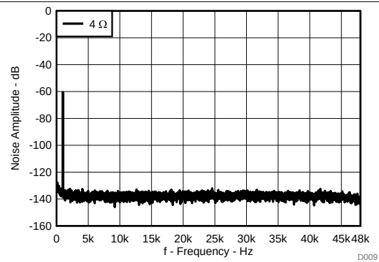
⊠ 12. Noise vs Frequency
