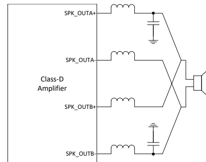
Figure 40. Post-Filter PBTTL
