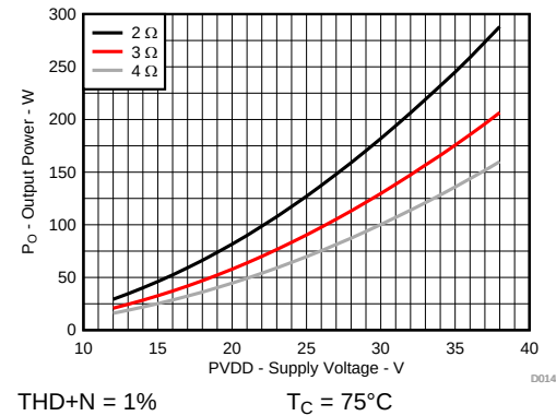
FIG 16. Output Power vs Supply Voltage
