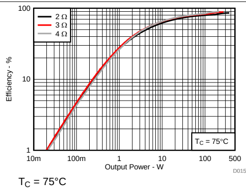
FIG 17. Efficiency vs Output Power
