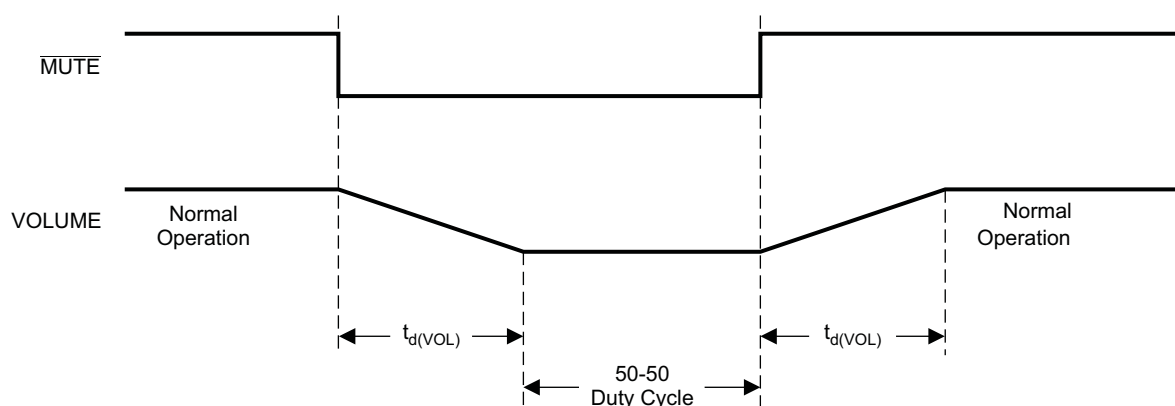
Figure 7. Mute Timing
