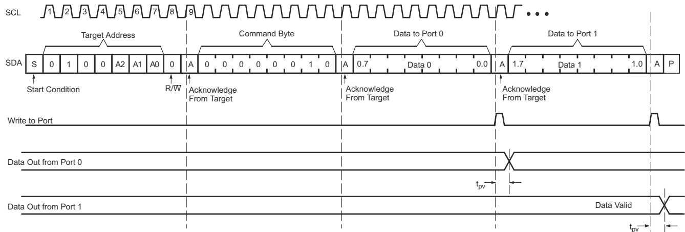
Fig 7-7. Write to Output Port Registers
