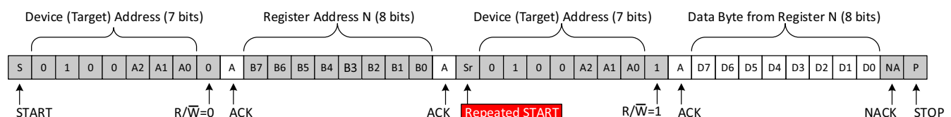
Fig 7-8. Read from Register
