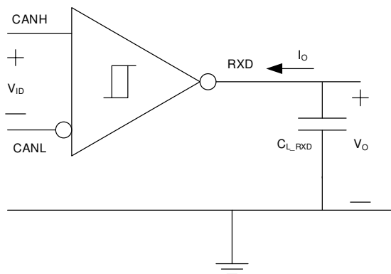
図 6-3. Receiver Test Circuit and Measurement
