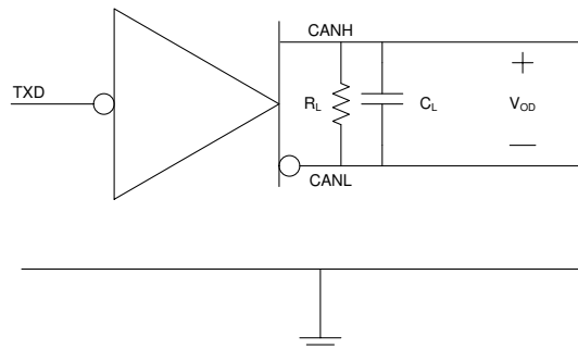
Figure 6-6. TXD Dominant Timeout Test Circuit and Measurement
