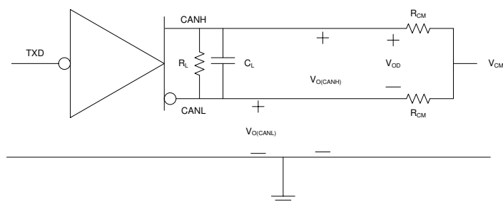
図 6-2. Driver Test Circuit and Measurement
