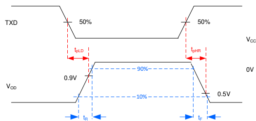
図 6-2. Driver Test Circuit and Measurement
