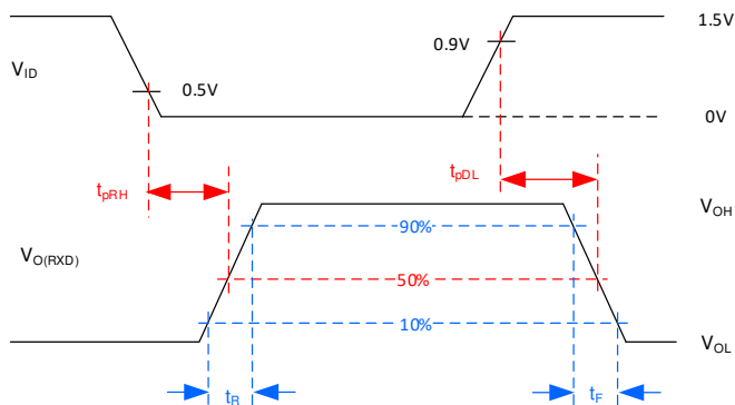
図 6-3. Receiver Test Circuit and Measurement
