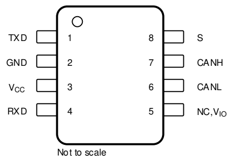
図 4-2. D Package, 8-Pin SOIC (Top View)
