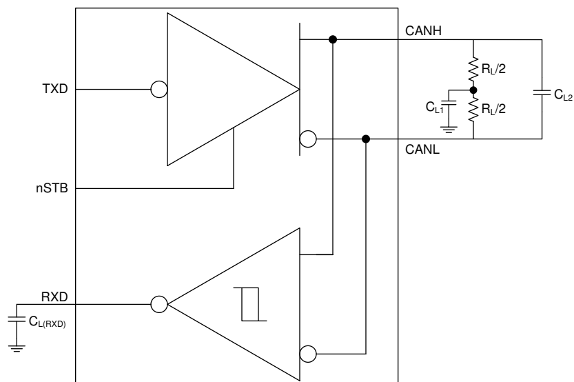
8-2. Test Circuit
