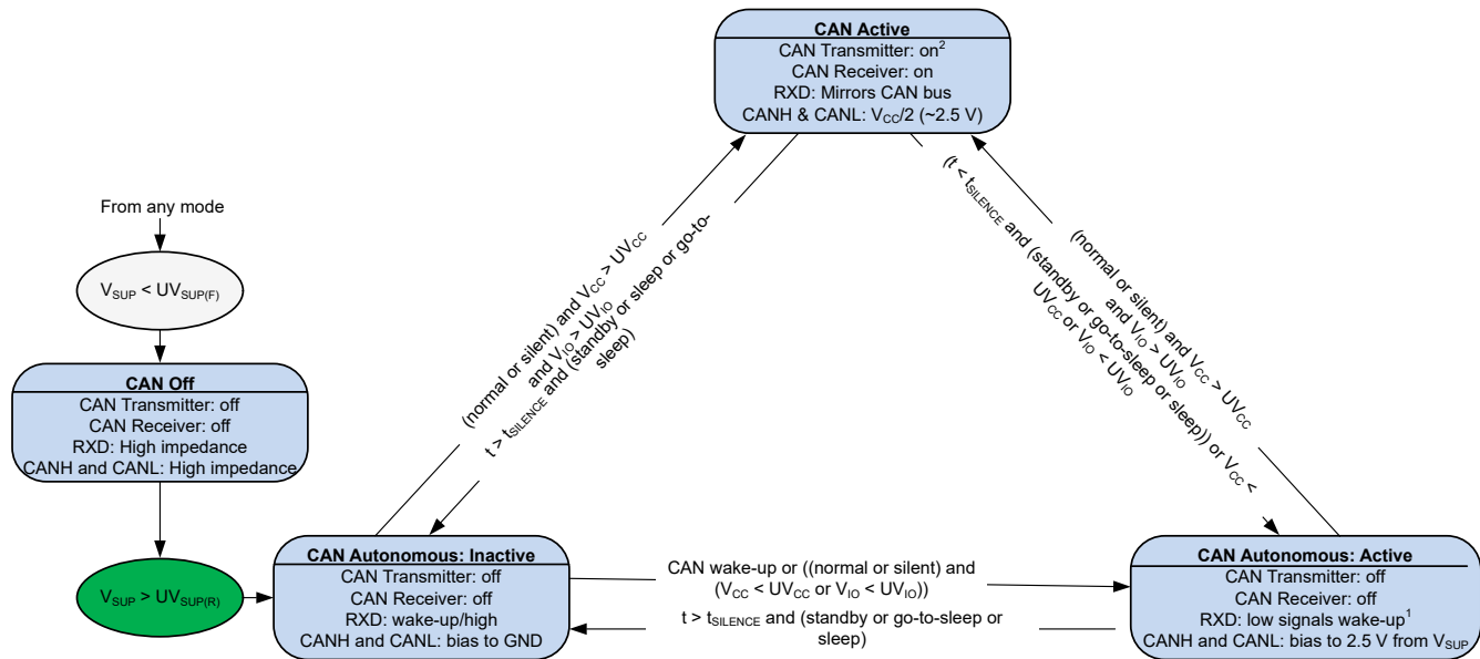
9-12. TCAN1463-Q1 CAN Transceiver State Machine
