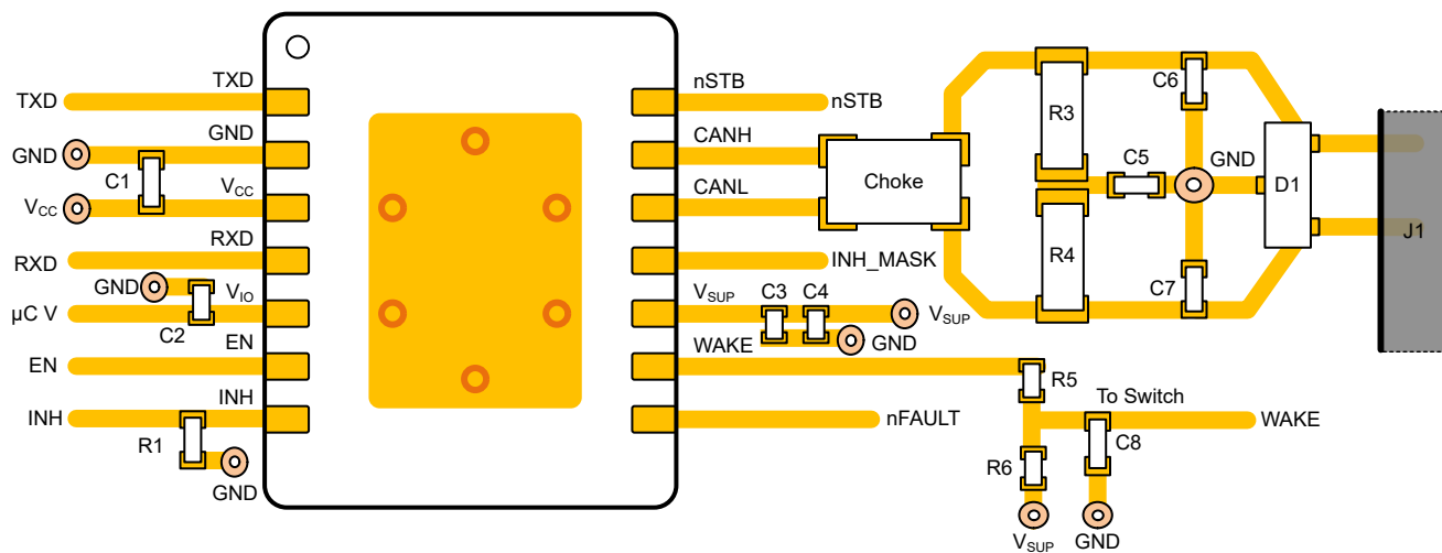
10-5. Example Layout
