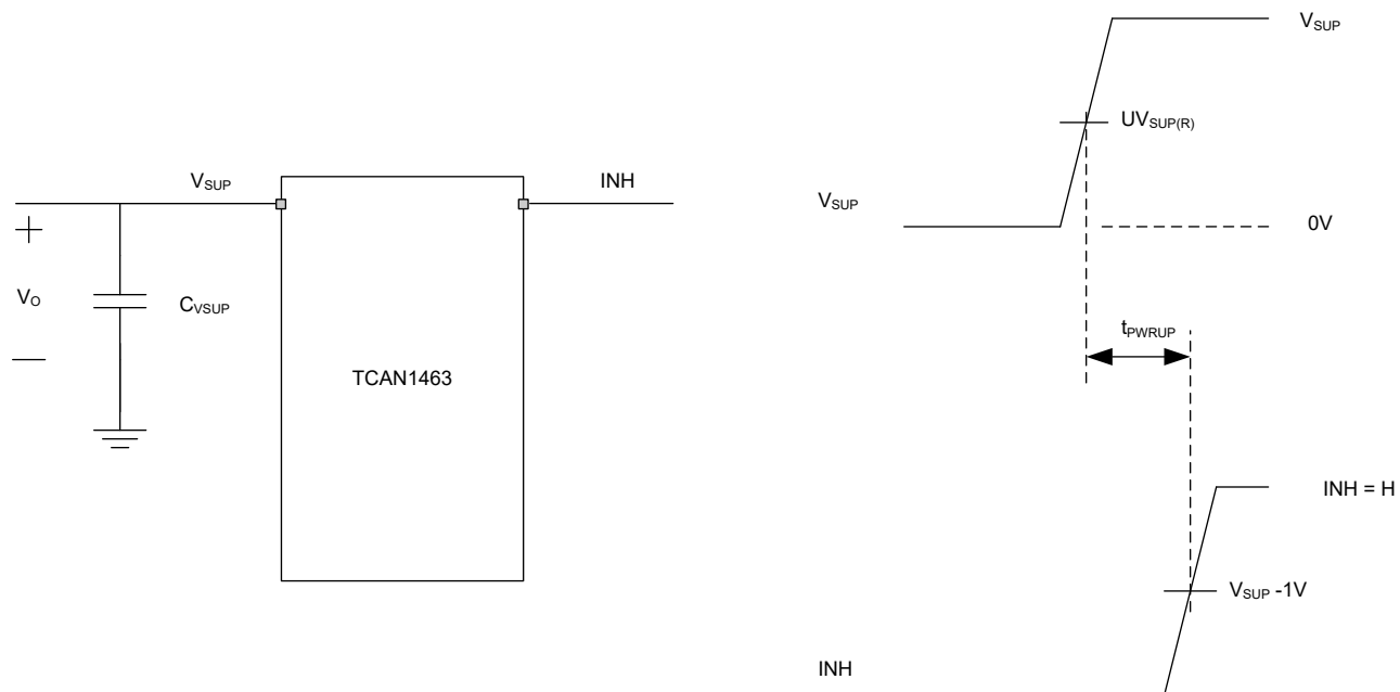
8-12. Power-Up Timing
