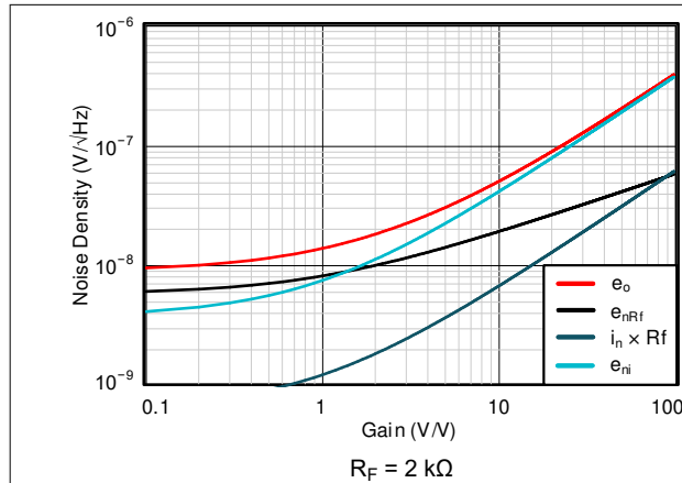
Figure 9-5. Calculated Noise Densities vs Gain Settings
