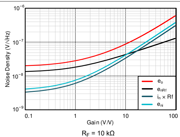
Figure 9-6. Calculated Noise Densities vs Gain Settings
